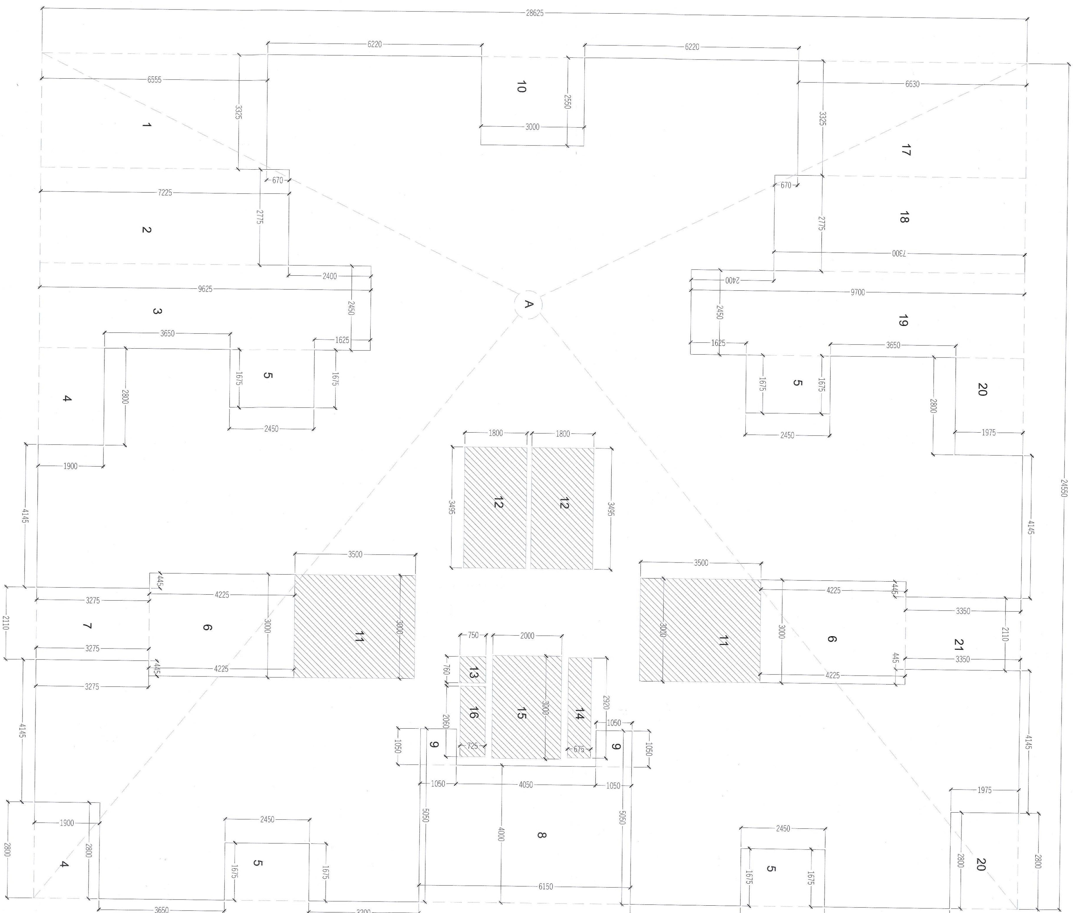
TYPICAL FLOOR FAR AREA DIAGRAM
