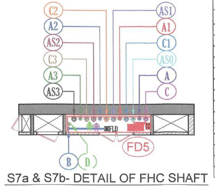
S7a & S7b- DETAIL OF FHC SHAFT
