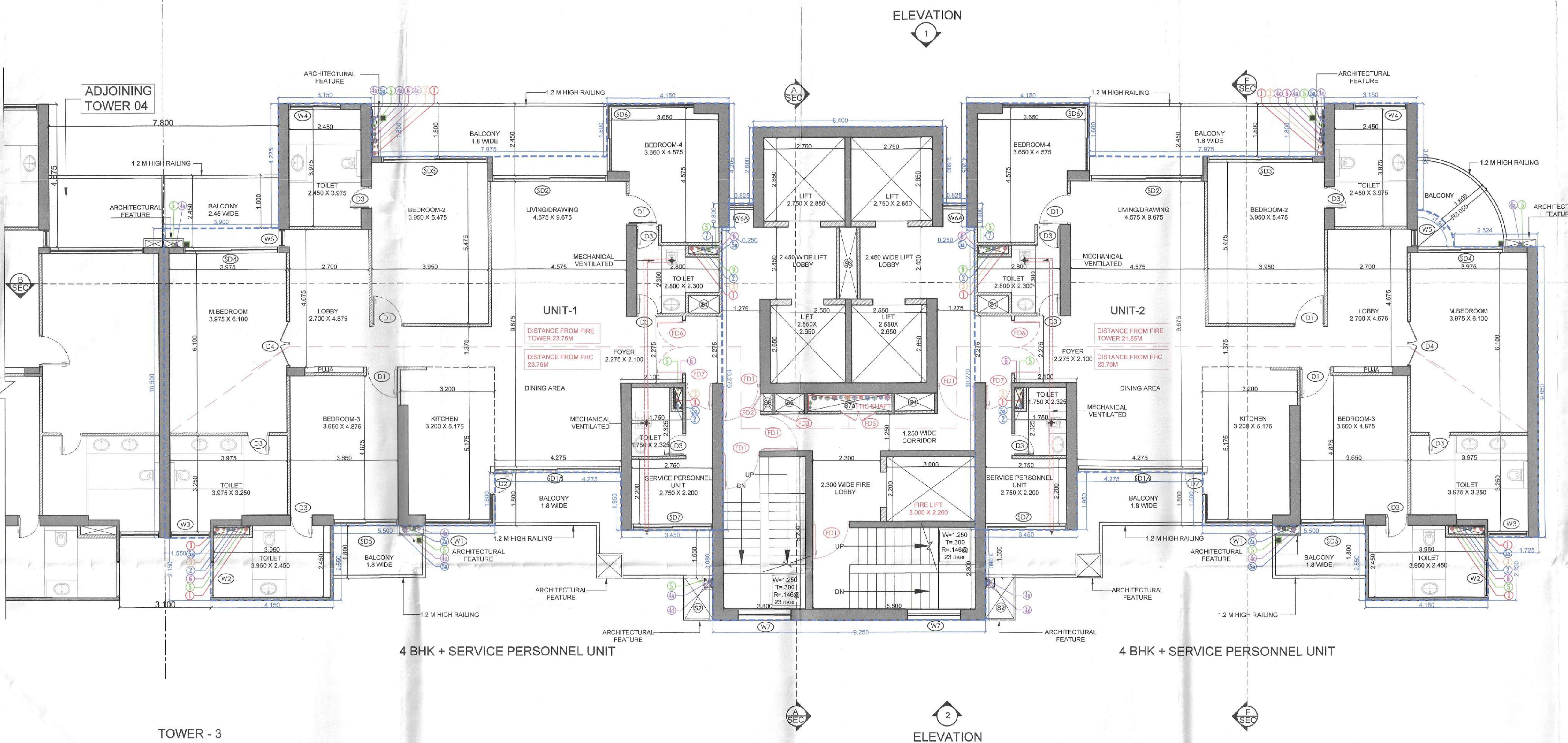
TOWER - 3 TYPICAL LVL LAYOUT (LEVEL-2ND (LVL +15.825 M) to 15th, 17th to 23rd, 25th to 32nd, 34th to 37th (vl +13.950 M) FLOOR
