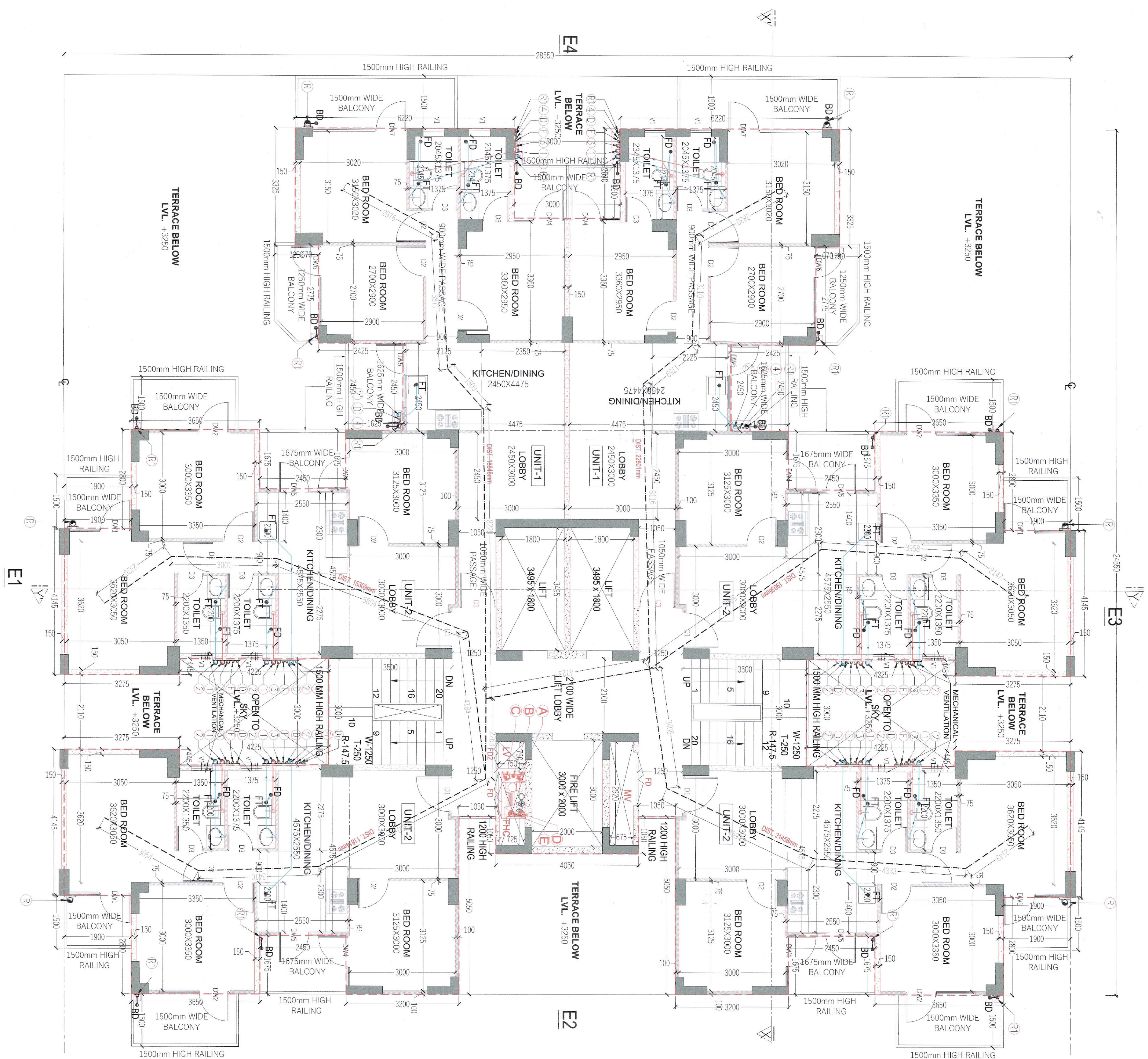
TYPICAL FLOOR PLAN 2ND TO 18th TOWER-H
