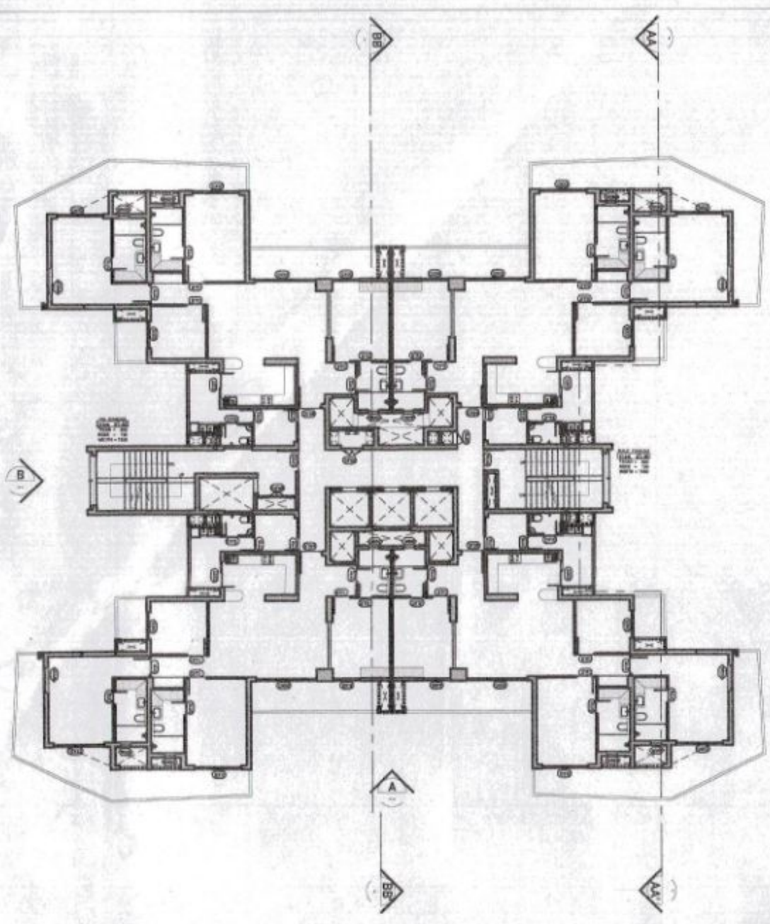
KEY PLAN, TYPICAL FLOOR
