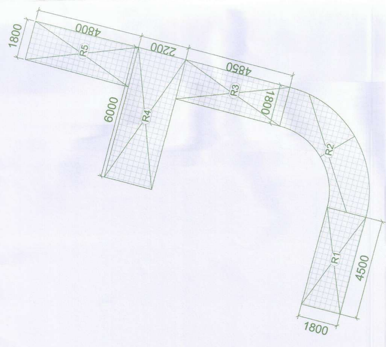
3. REFUGE AREA DIAGRAM SCALE: 1:100
