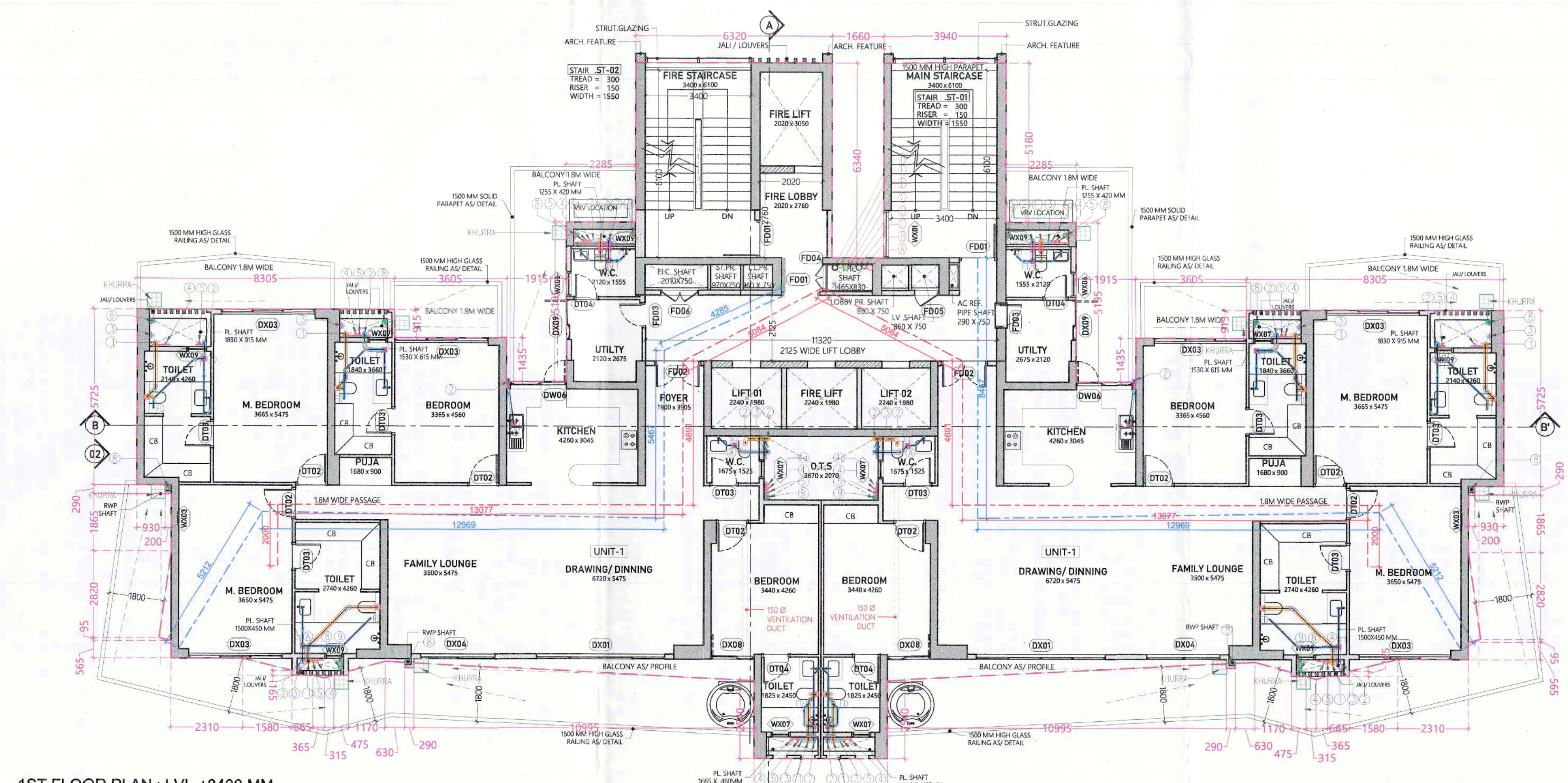
1ST FLOOR PLAN; LVL +8400 MM
