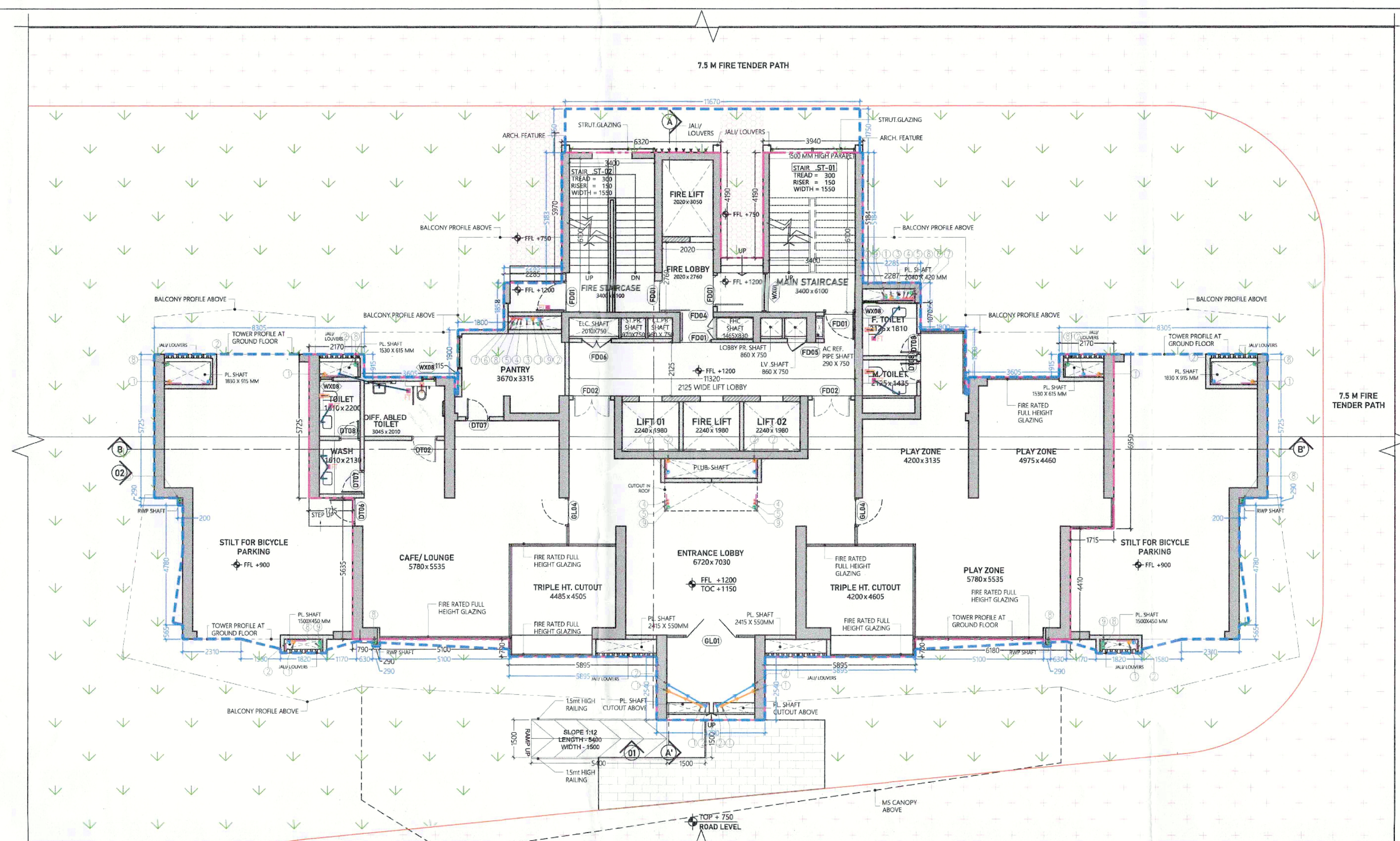
STILT FLOOR / GROUND FLOOR PLAN LVL +1200 MM
