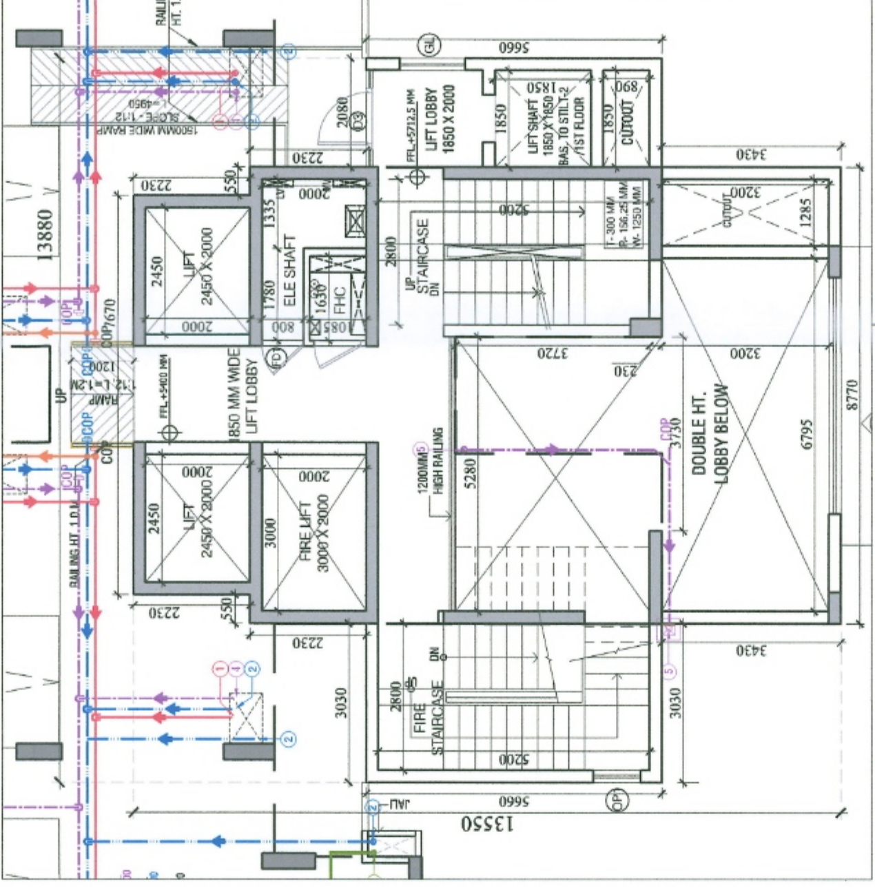
DETAIL-1 TYPE-A, TOWER-4 & 6 (SCALE:1:100)
