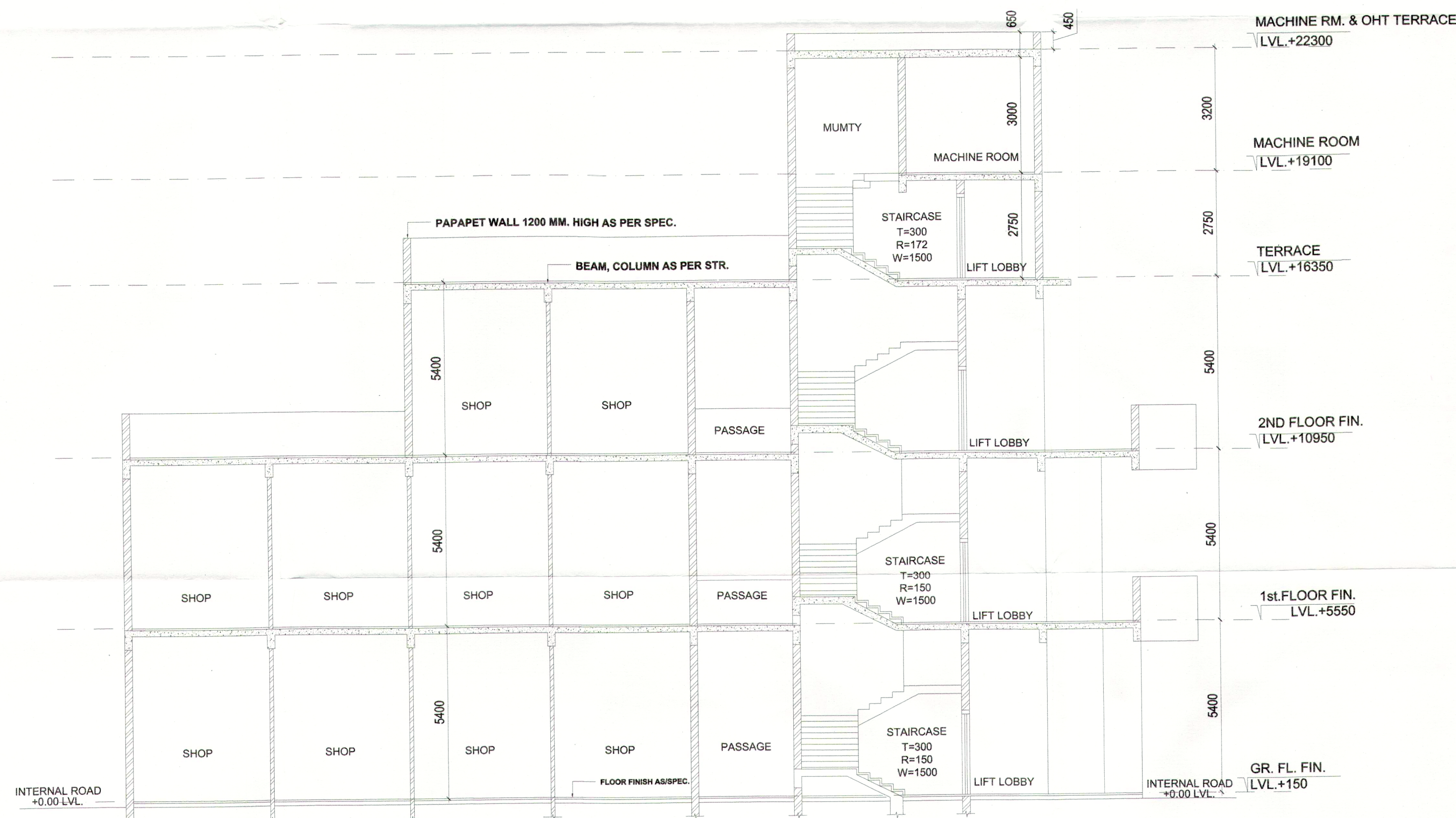
SECTION - BB
