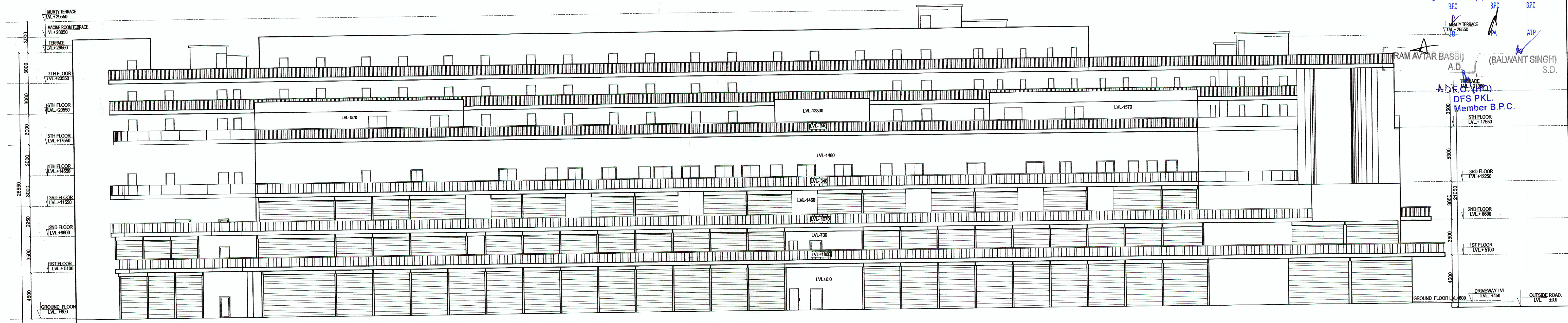
ELEVATION-1
