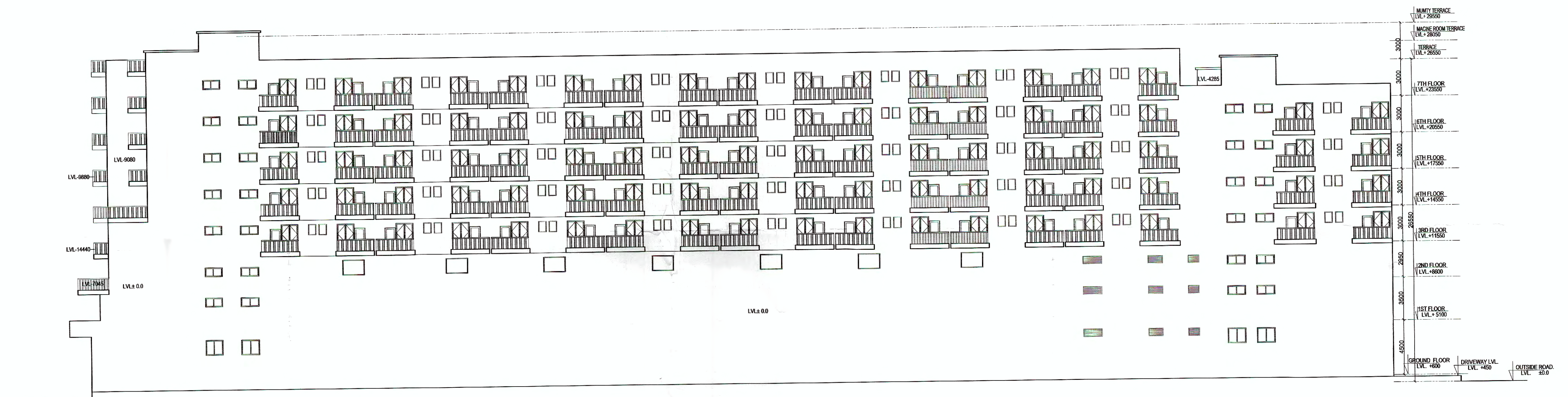
ELEVATION AT 3
