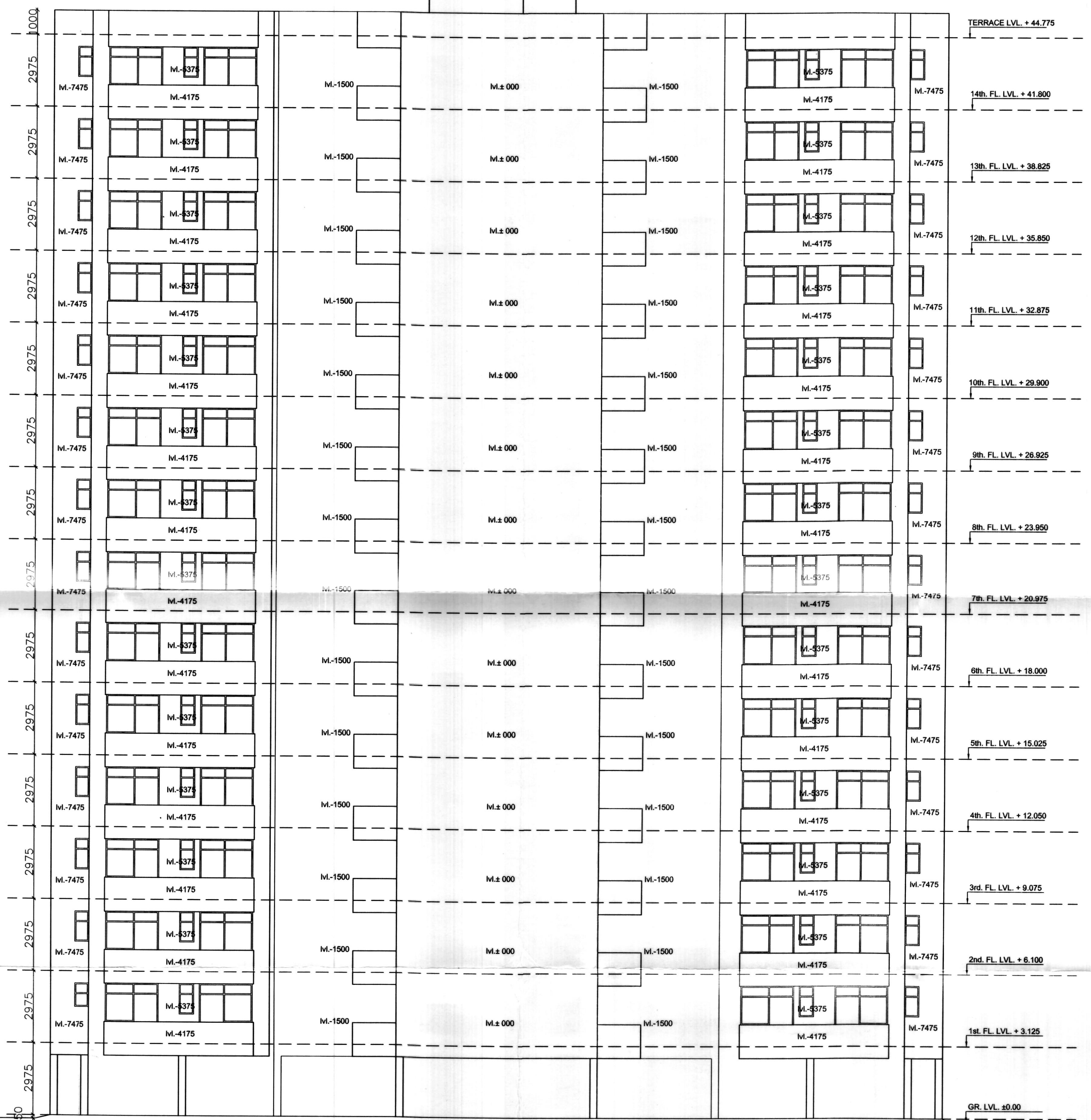
ELEVATION -2
