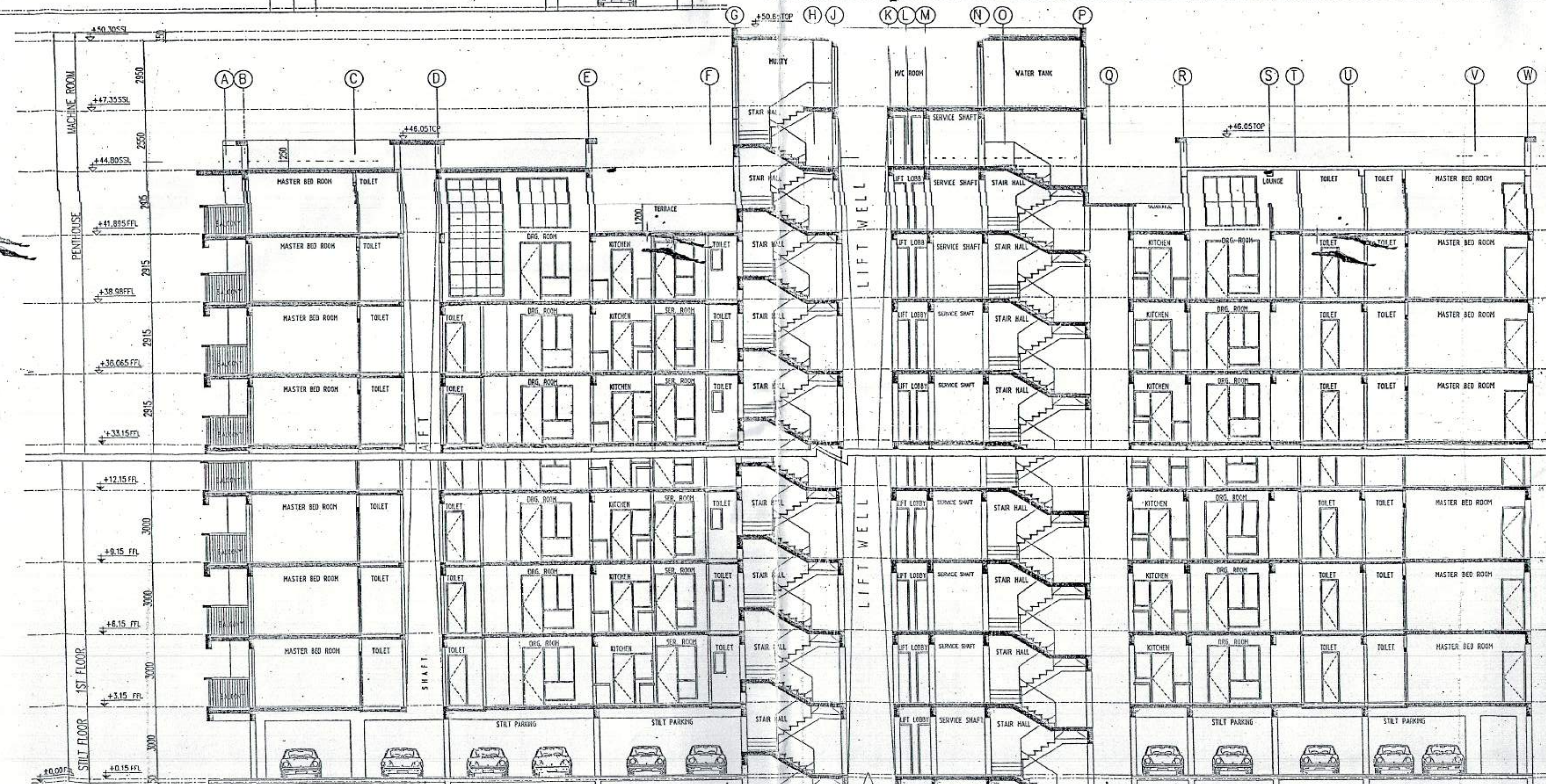
SECTION - S1 (SCALE 1:100)
