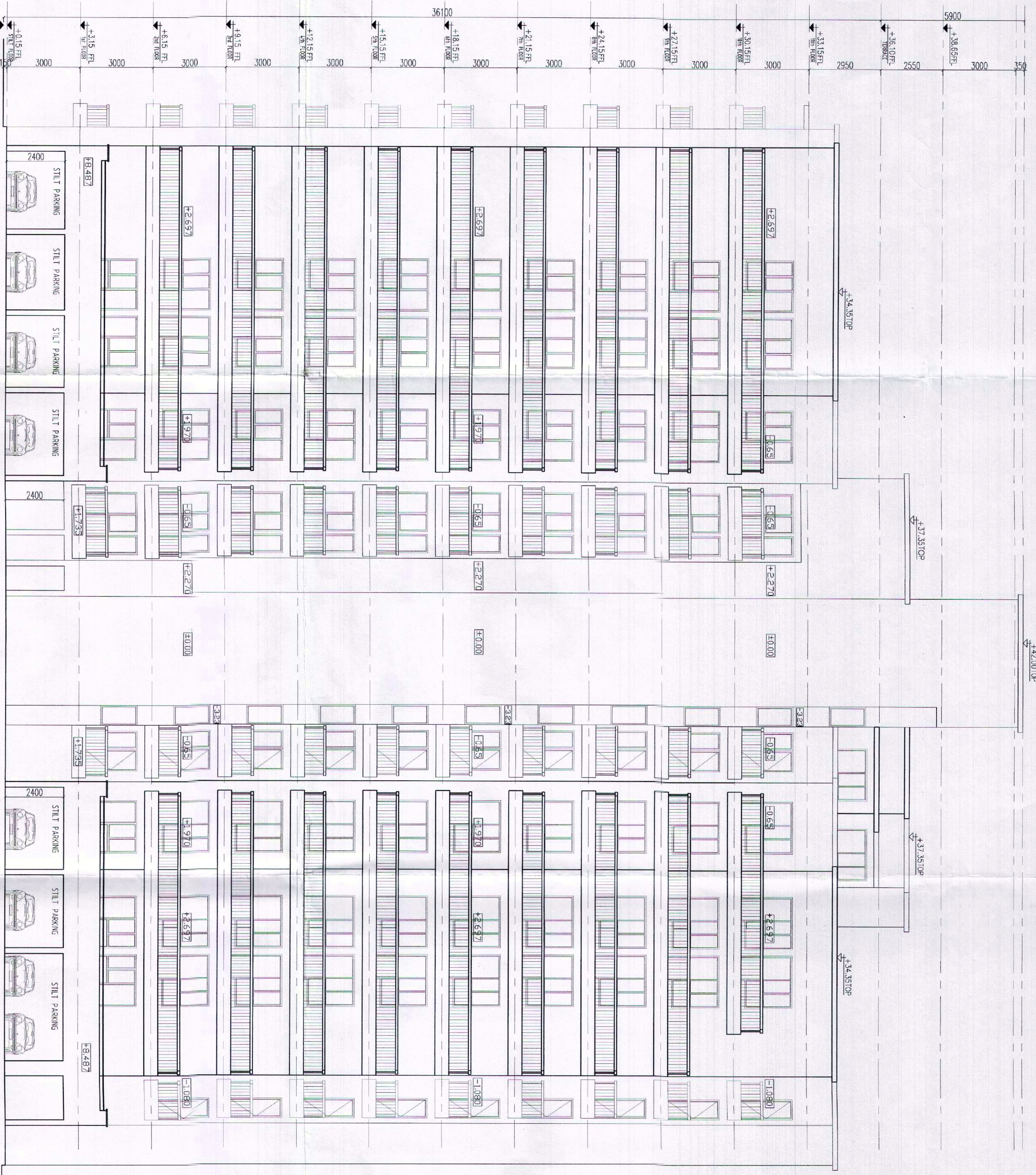
ELEVATION - 1 SCALE 1:100
