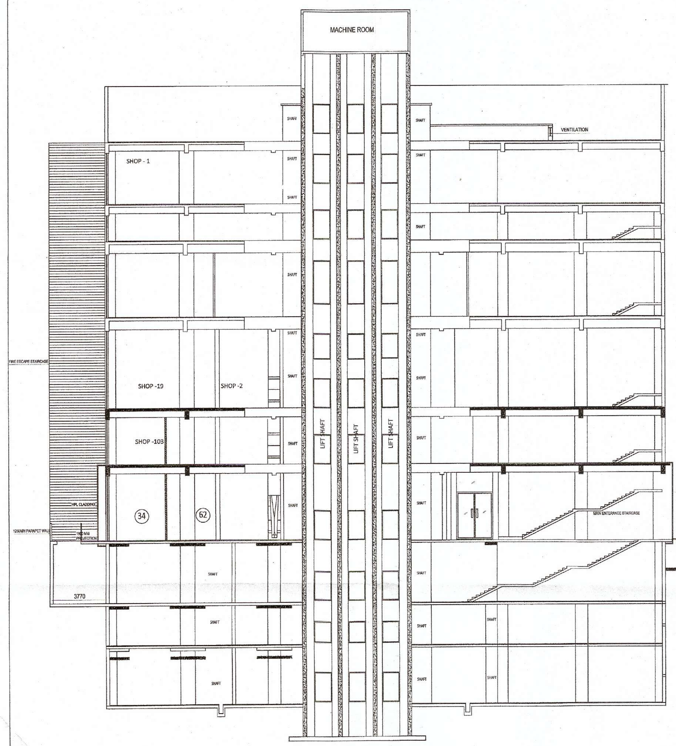
SECTION BB'
