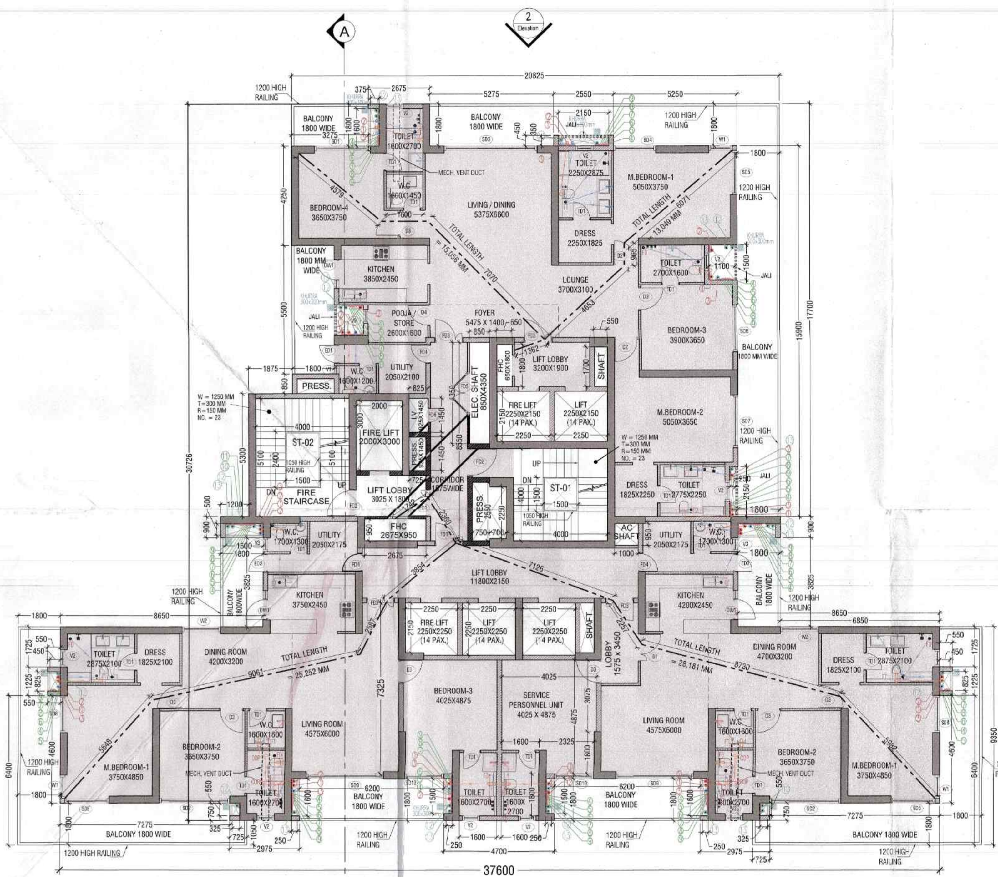
TYPICAL FLOOR PLAN (3th-16th, 18th-24th, 26th-33th, 35th-41st)
