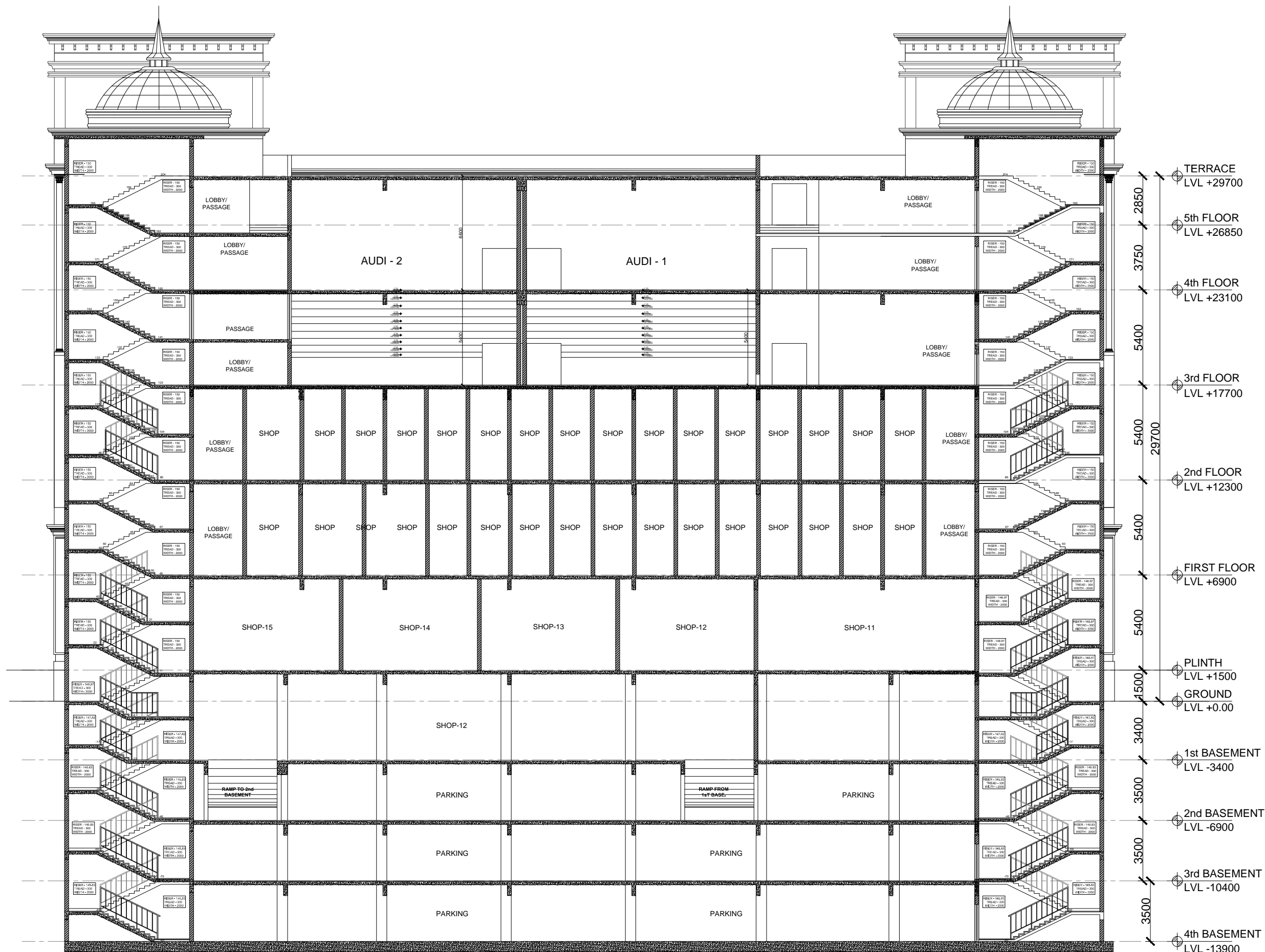
SECTION - BB'
