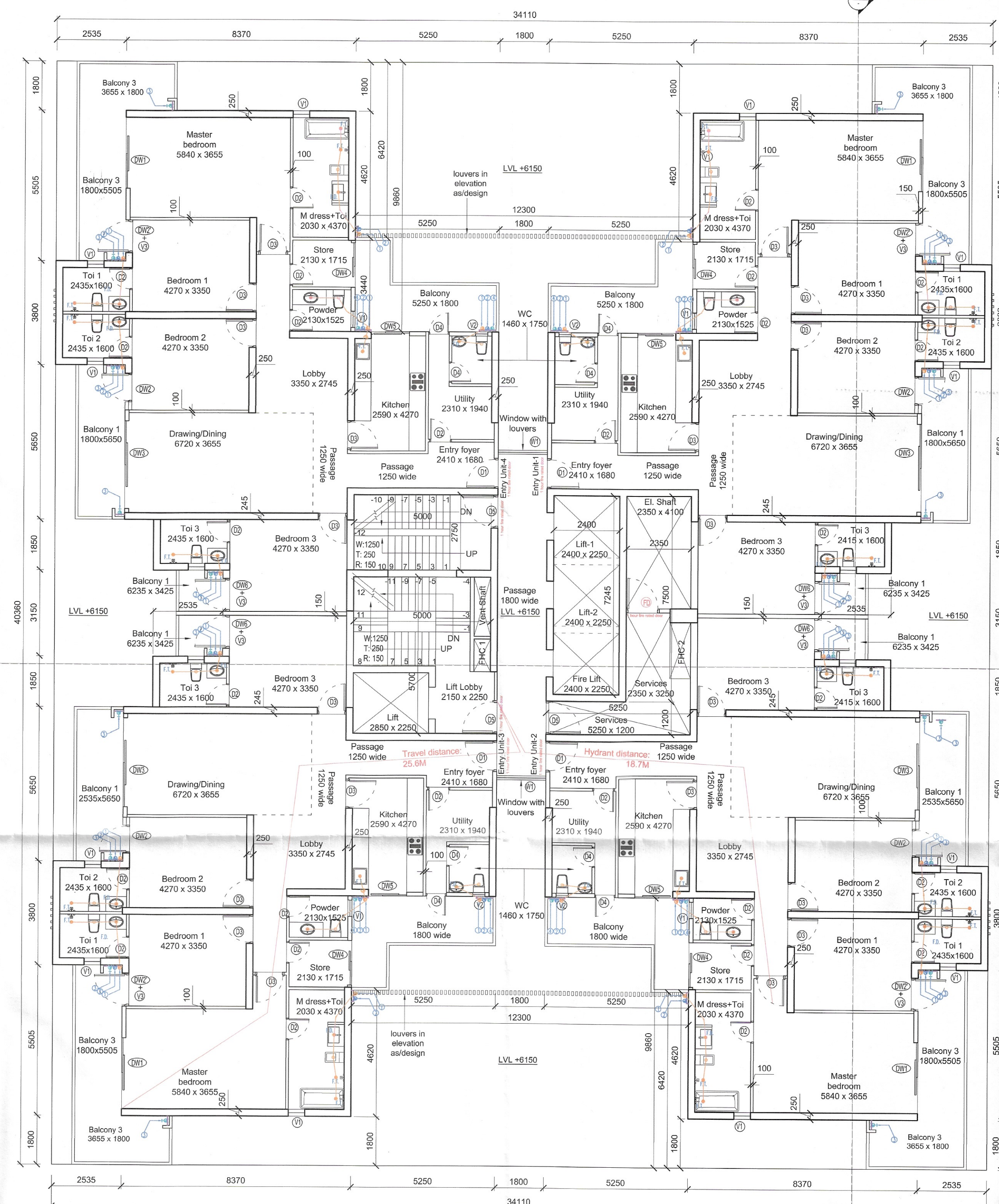
2 Type D- First Floor Plan SCALE - 1:110
