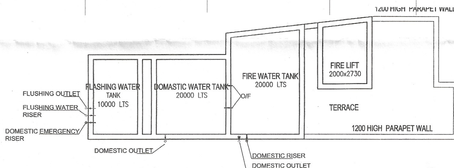
OVERHEAD WATER TANK PLAN
