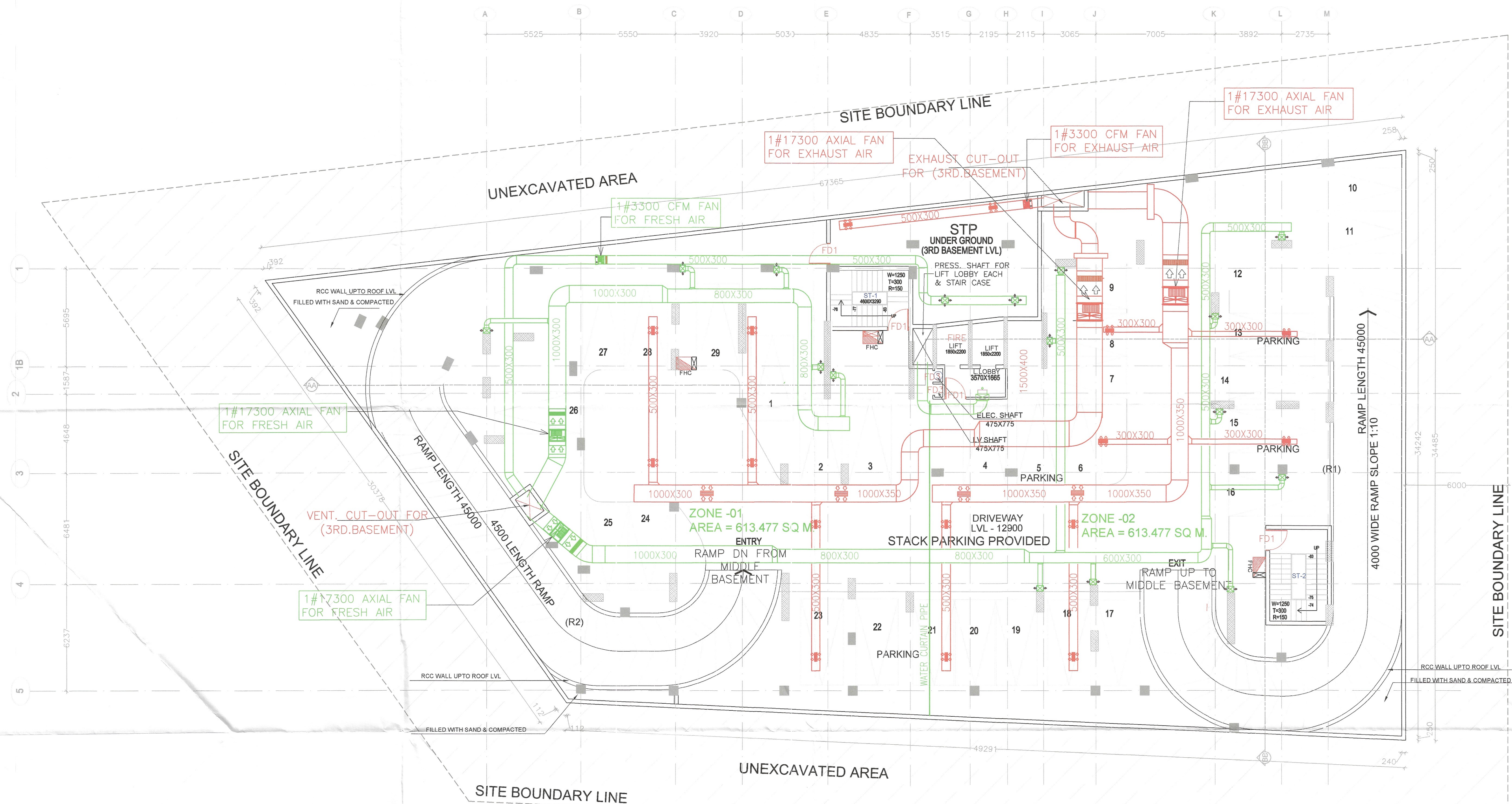
LOWER BASEMENT PLAN (VENTILATION SYSTEM)
