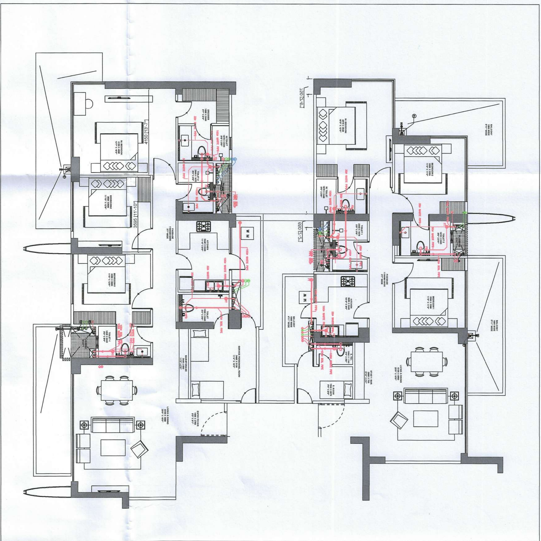
DRAINAGE
