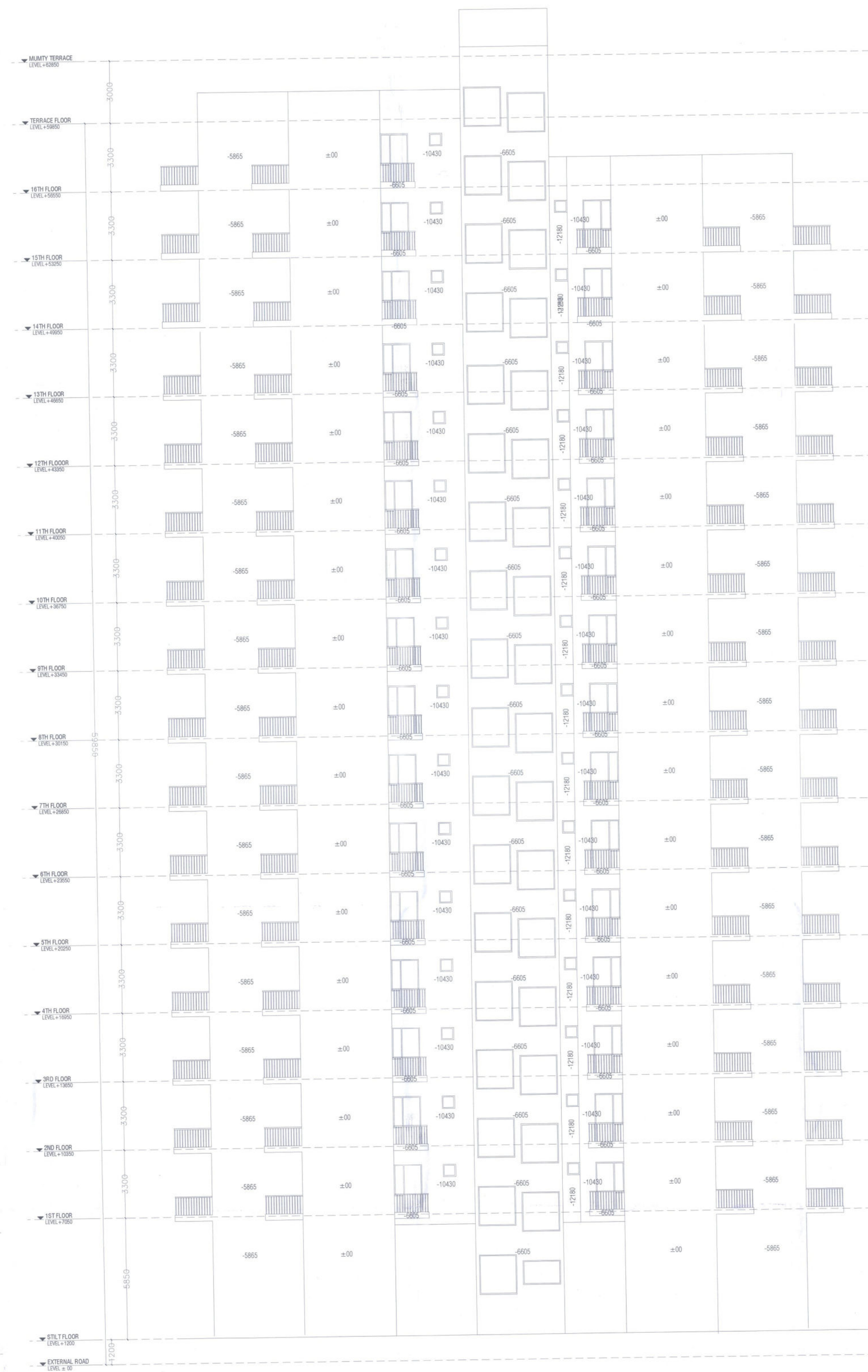
13 BUILDING ELEVATION AT A (TOWER TYPE-2A)
