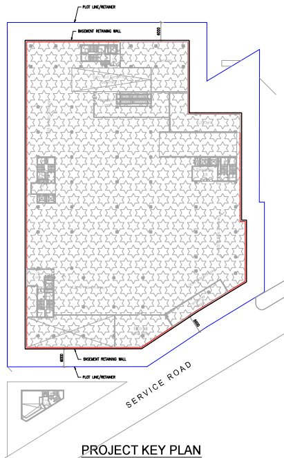
PROJECT KEY PLAN
