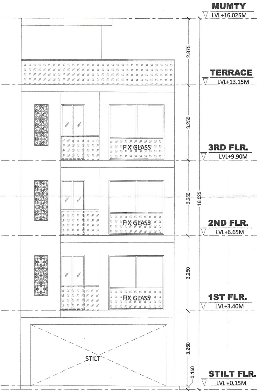
REAR ELEVATION
