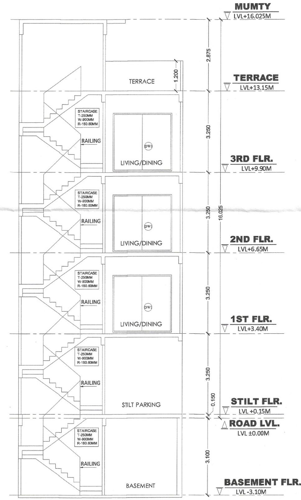
SECTION-B-B'
