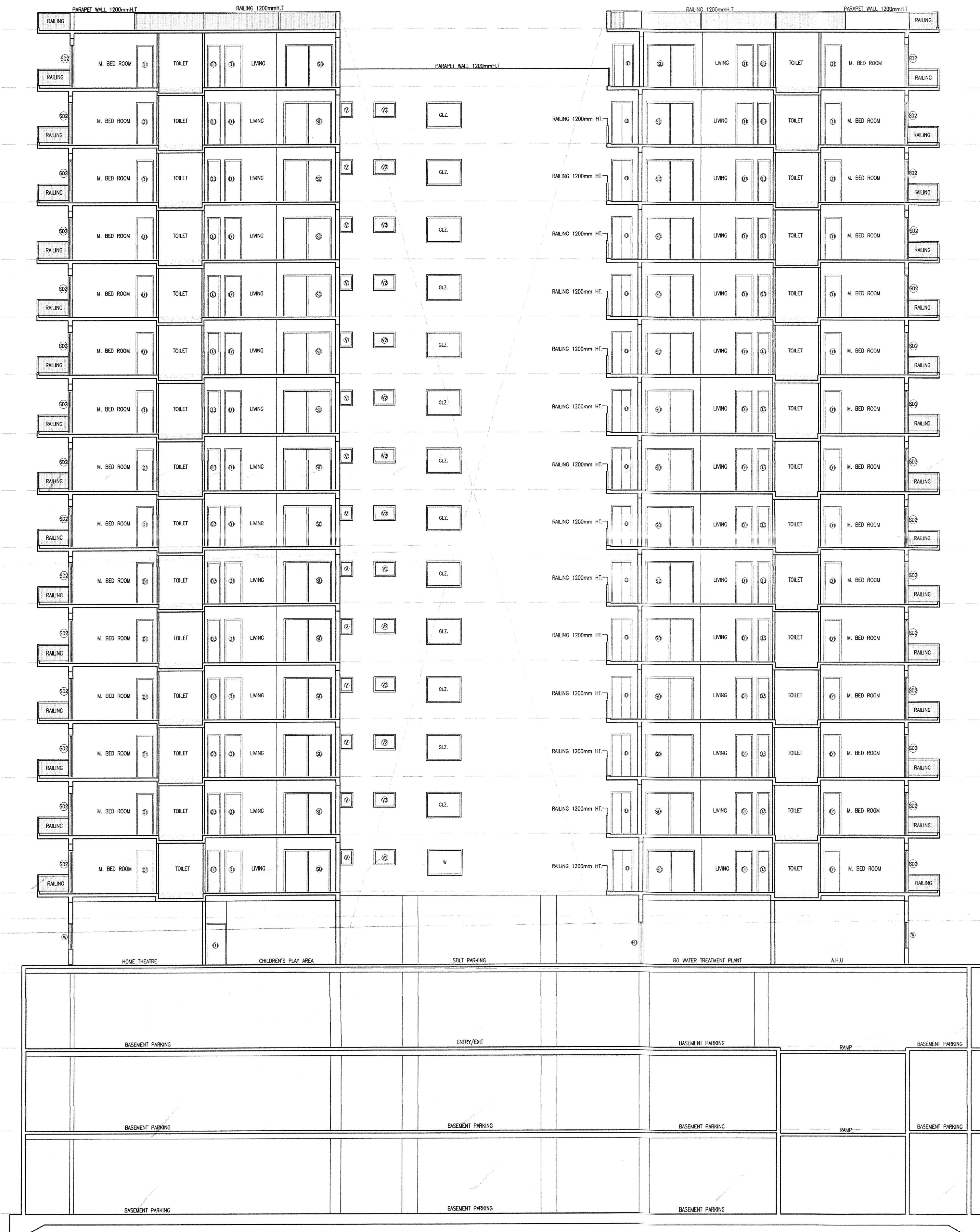
SECTION-A-A'
