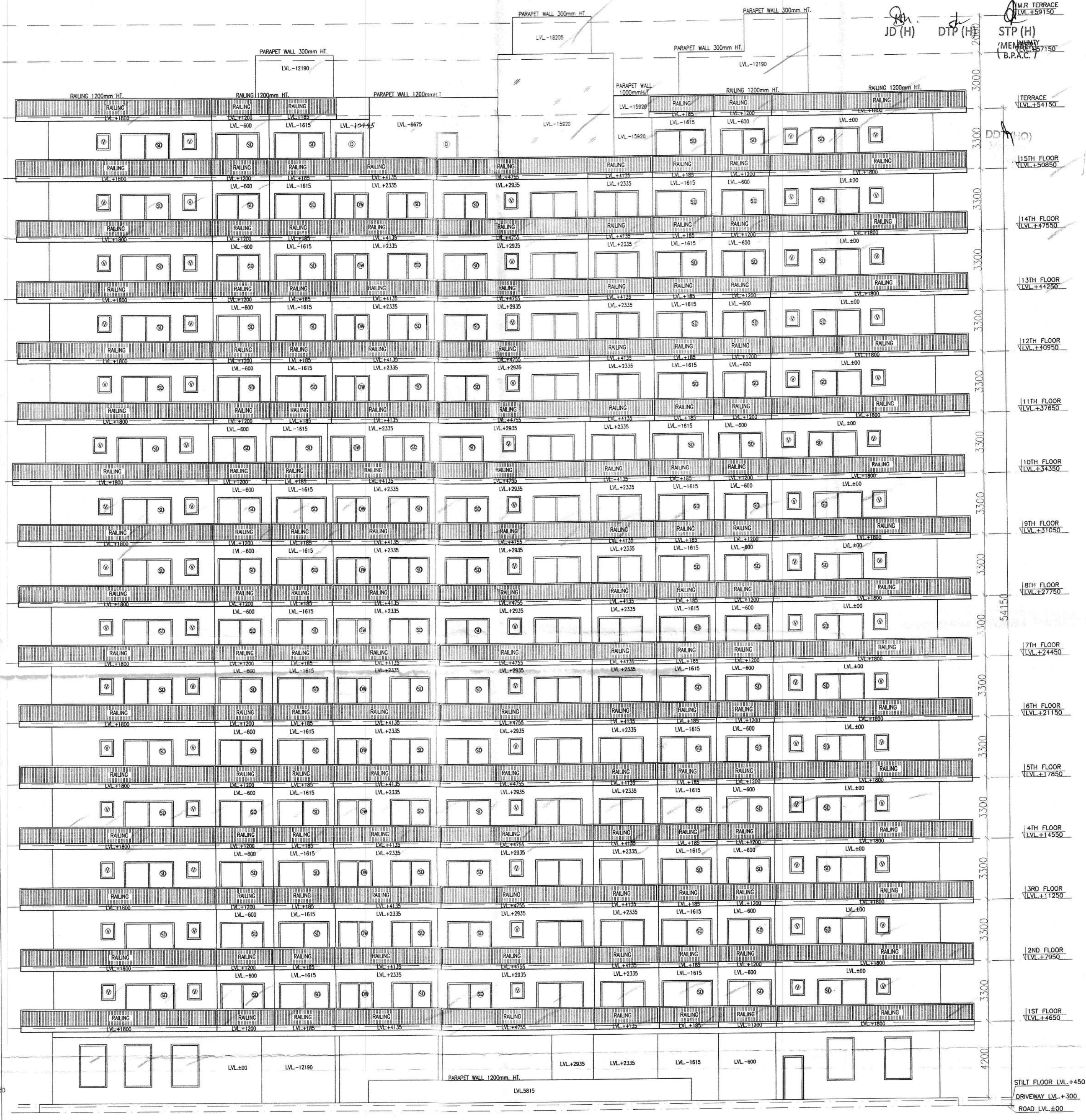
ELEVATION-B
