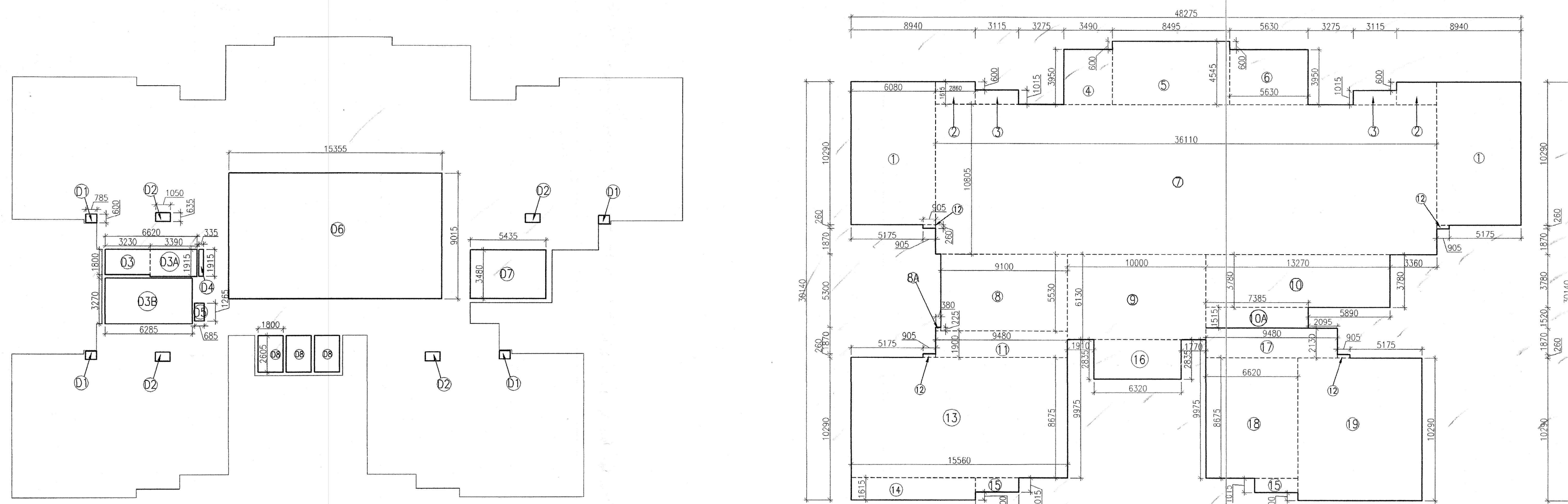
3RD FLOOR DEDUCTION AREA DIAGRAM (SCALE:- 1:200)
