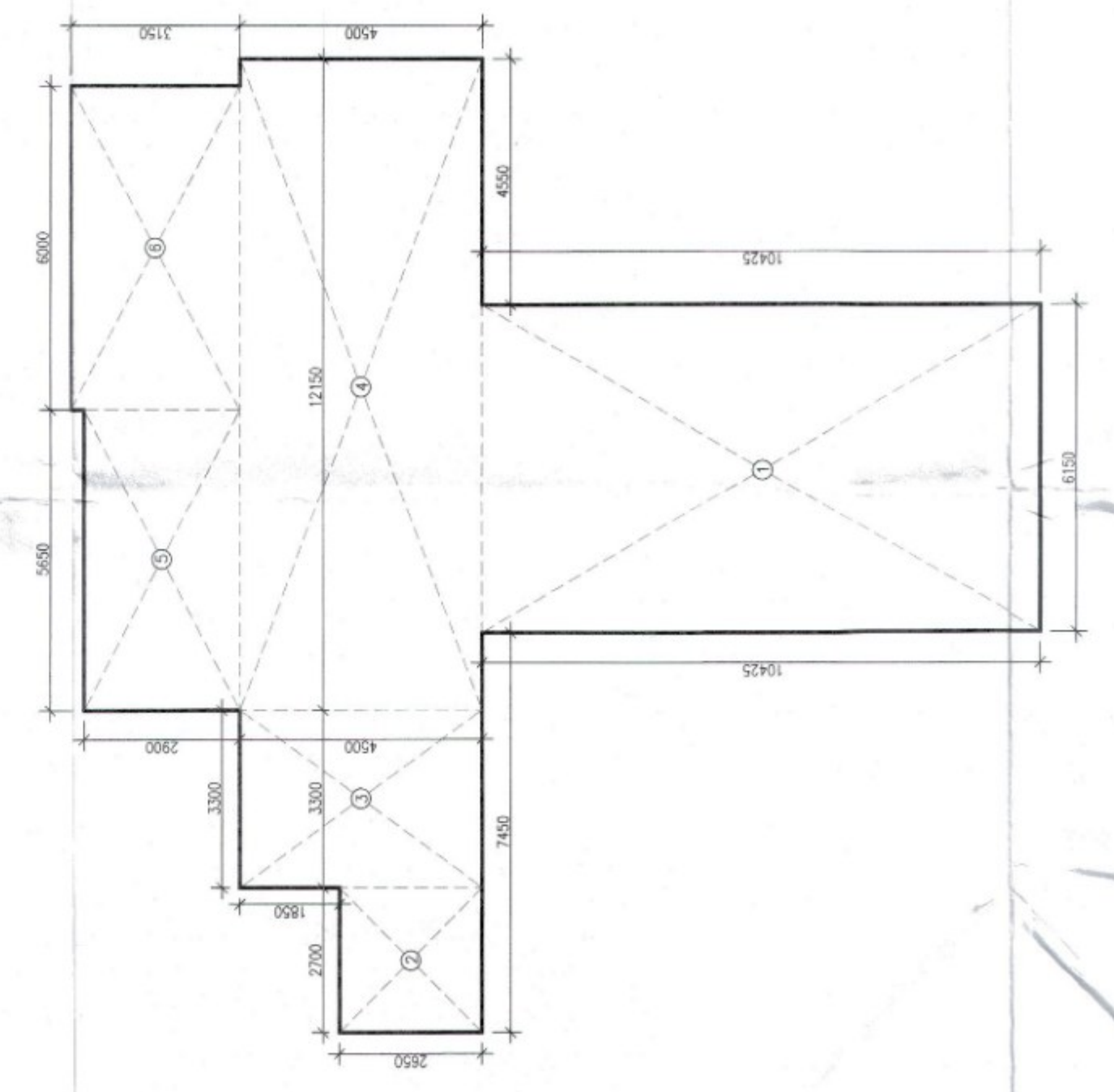
MUMMY & MACHINE ROOM AREA DIAGRAM TOWER-12
