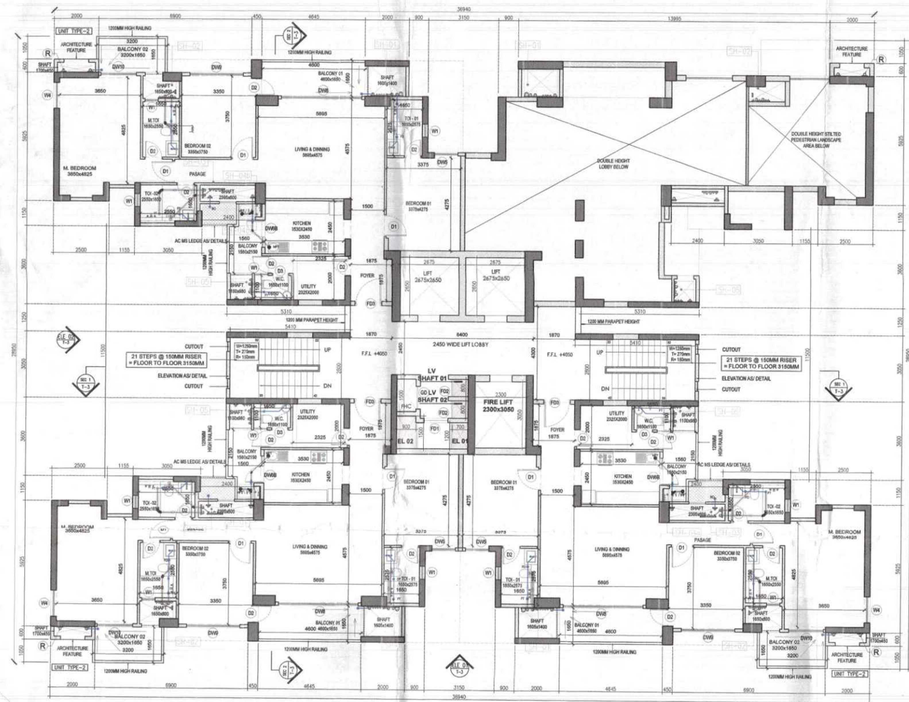
1 TOWER 3 - FIRST FLOOR PLAN 1:100
