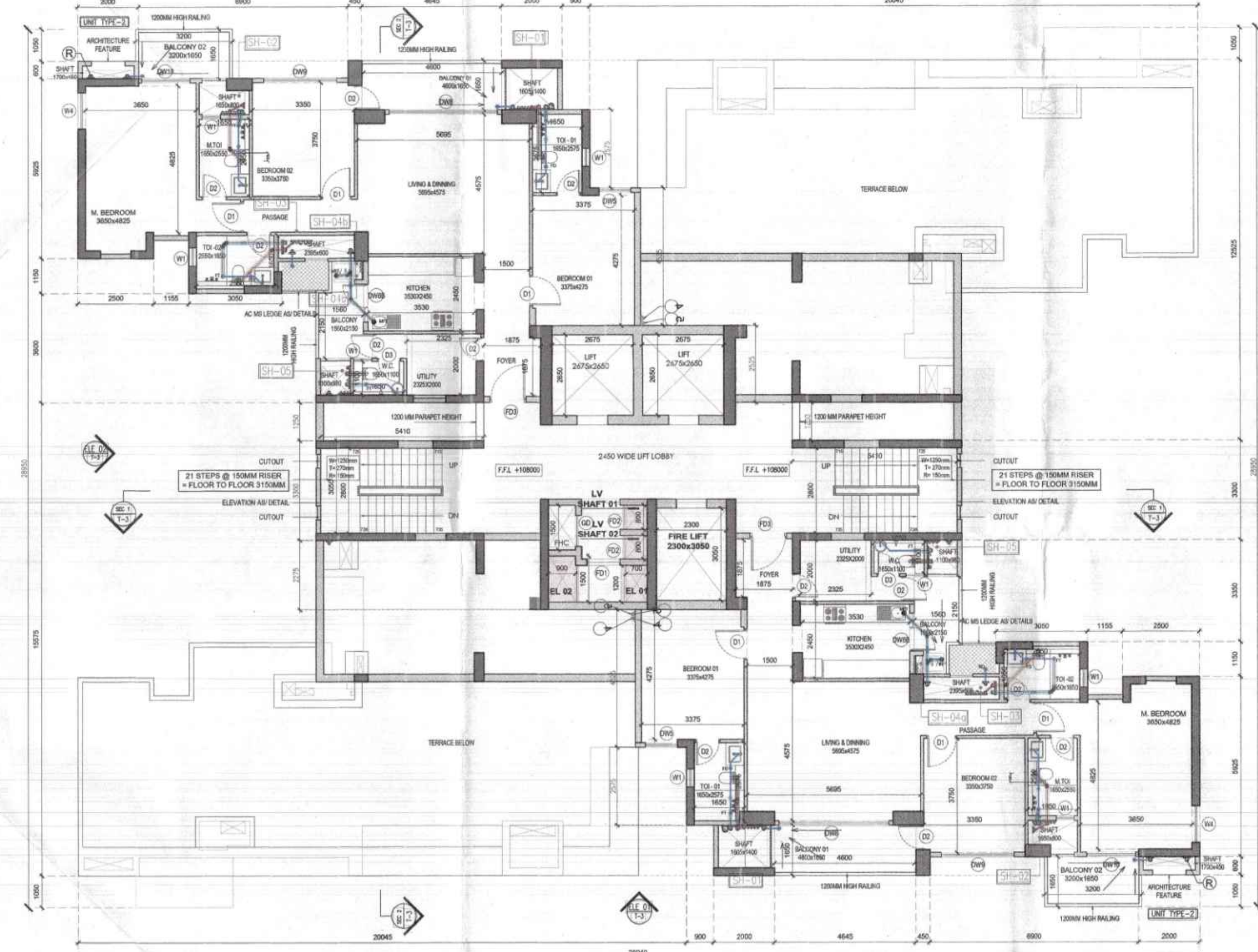
3 TOWER 3 - 34TH FLOOR PLAN 1:100
