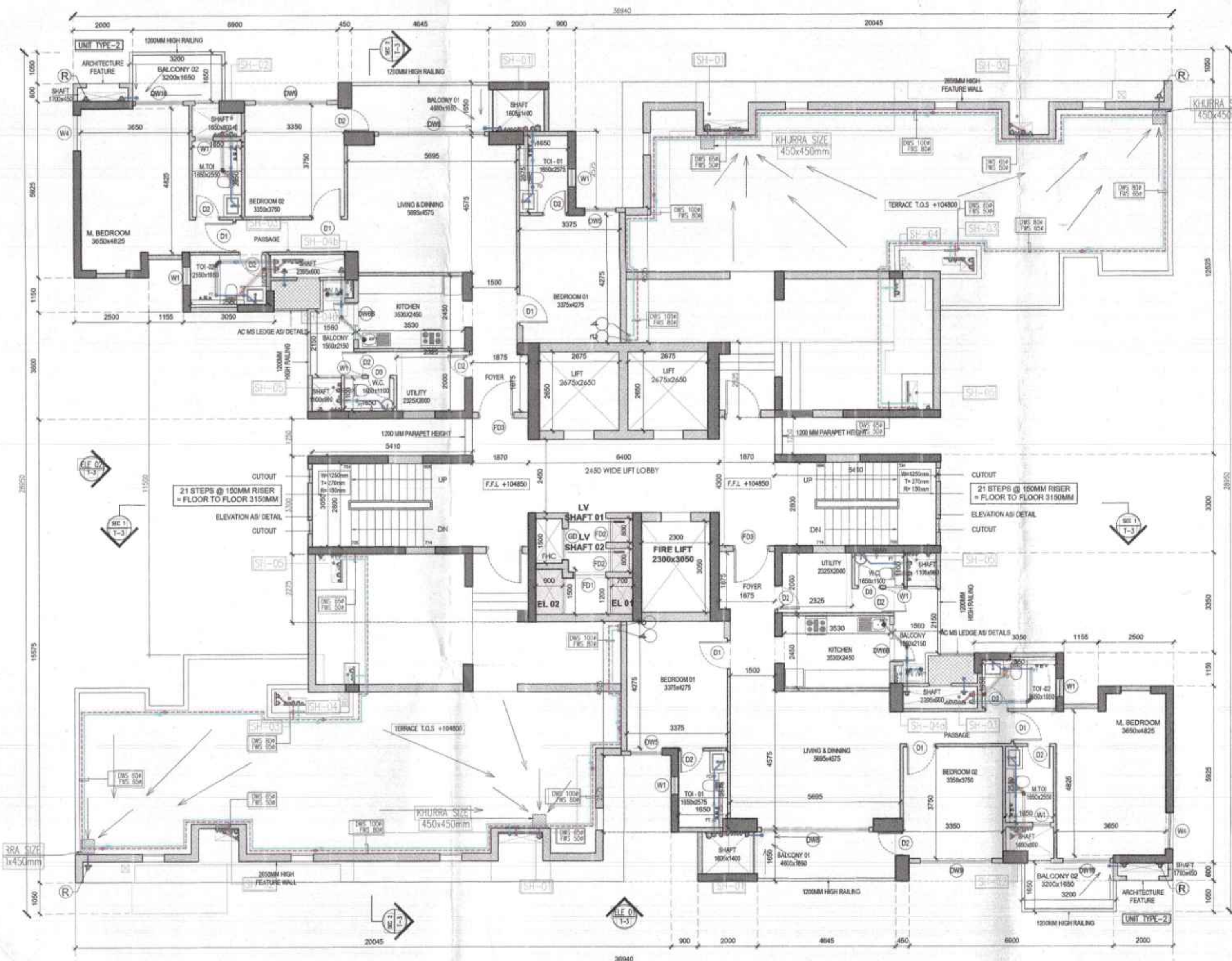
1 TOWER 3 - 33RD FLOOR PLAN 1:100
