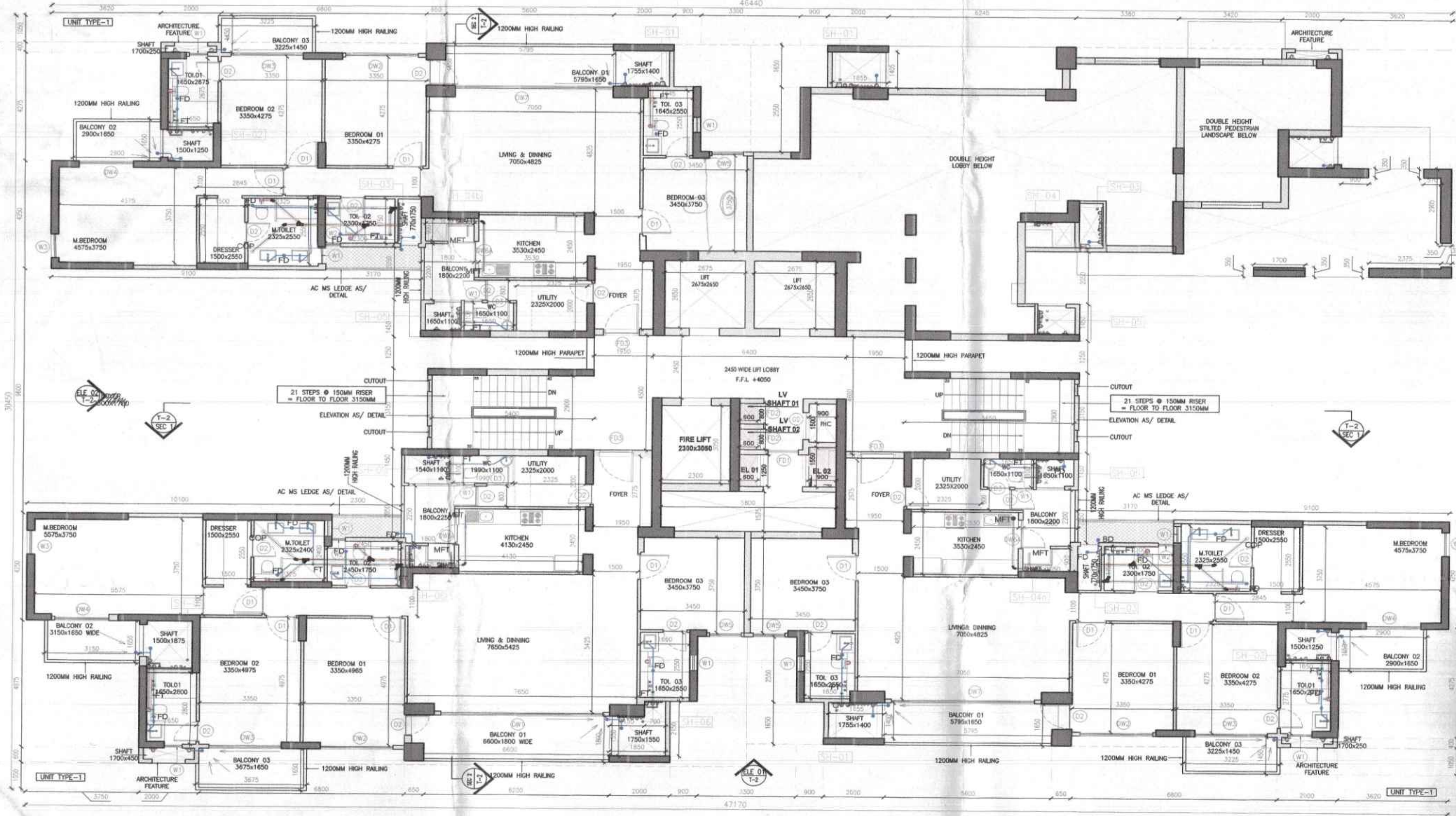
1 TOWER 2 - FIRST FLOOR PLAN 1:100
