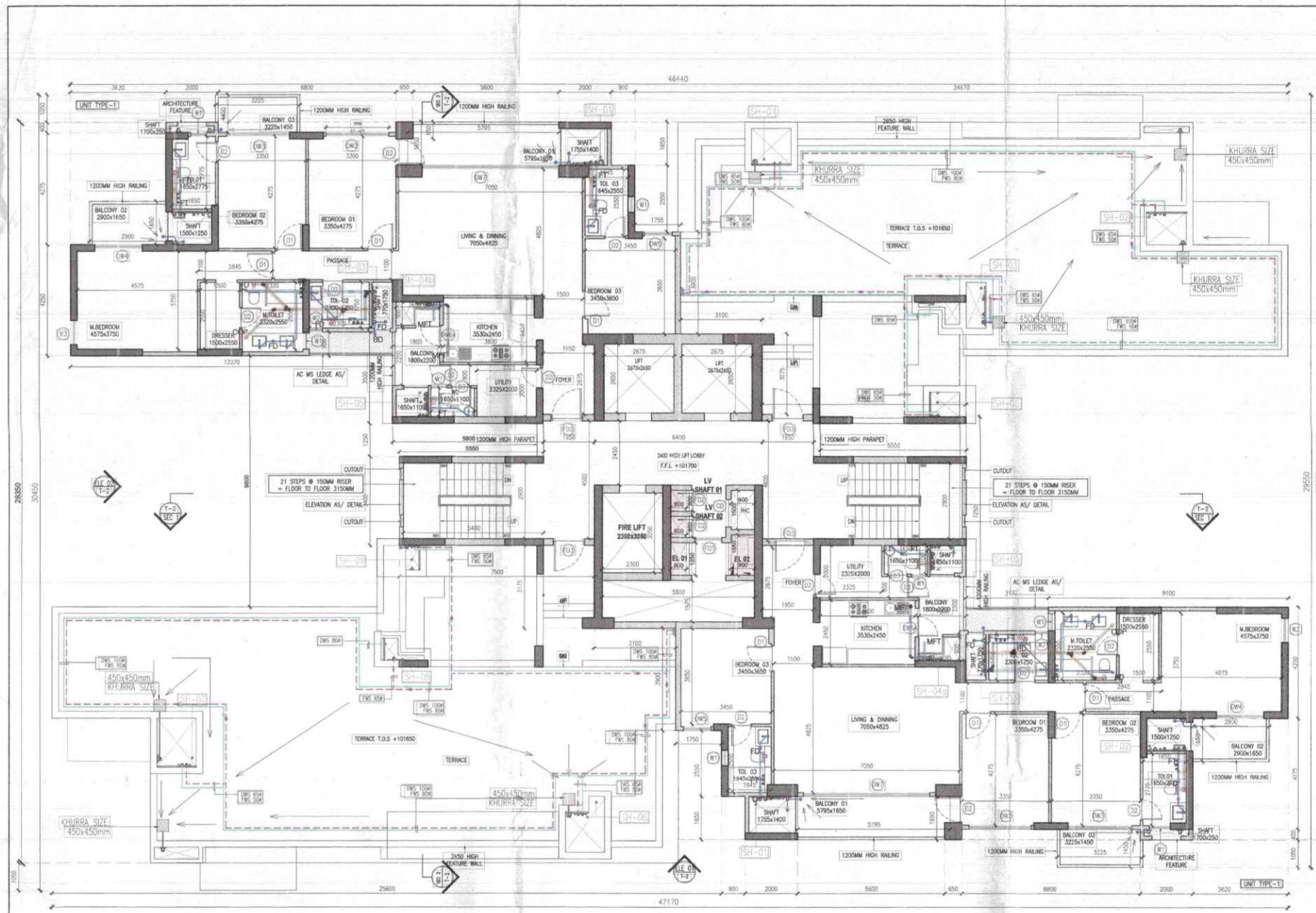
1 TOWER 2 - 32ND FLOOR PLAN 1:100
