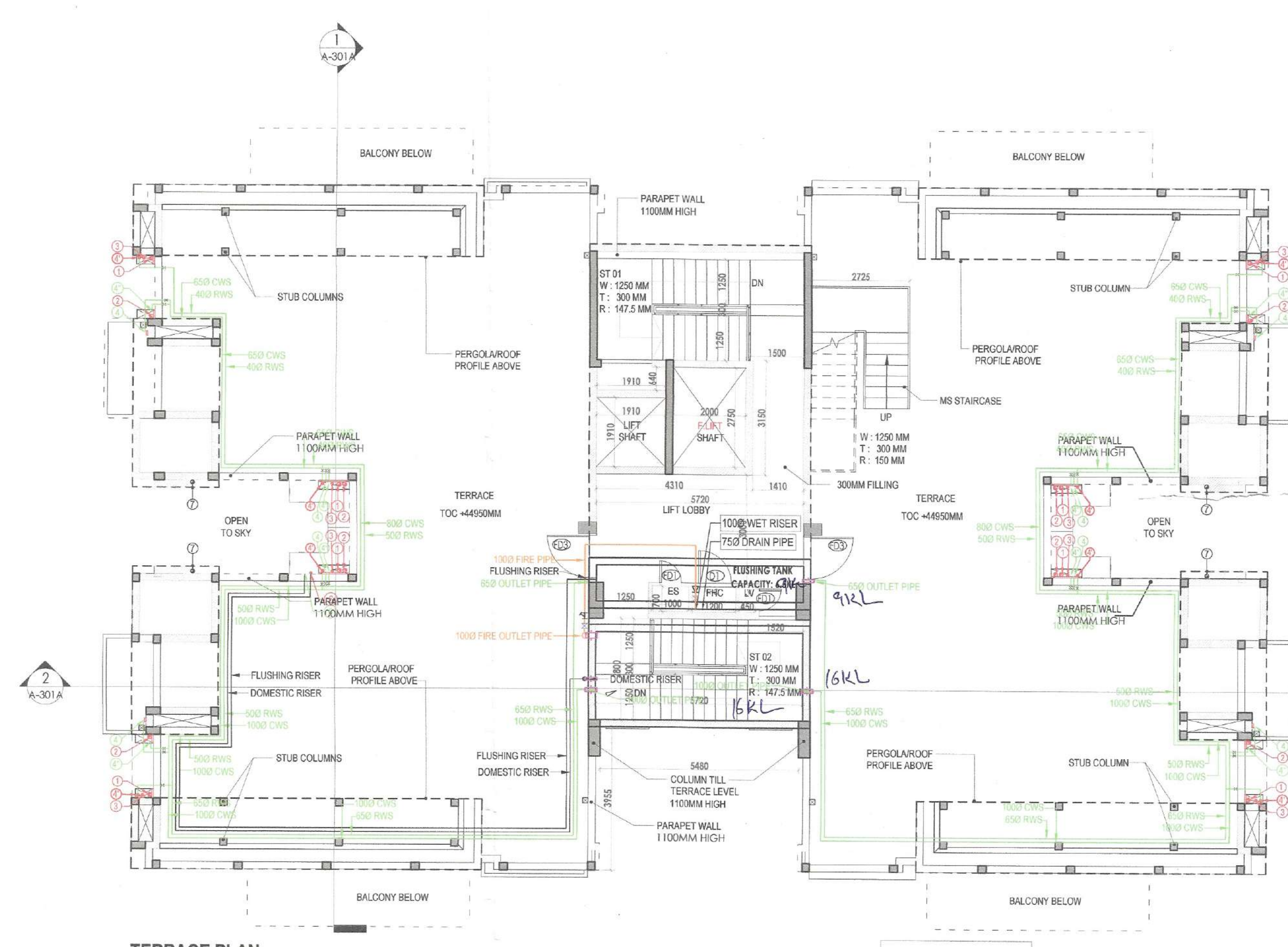
TERRACE PLAN TOWER - 1, 3, 6, 8, 11, 12, 14, 17, 19 & 21
