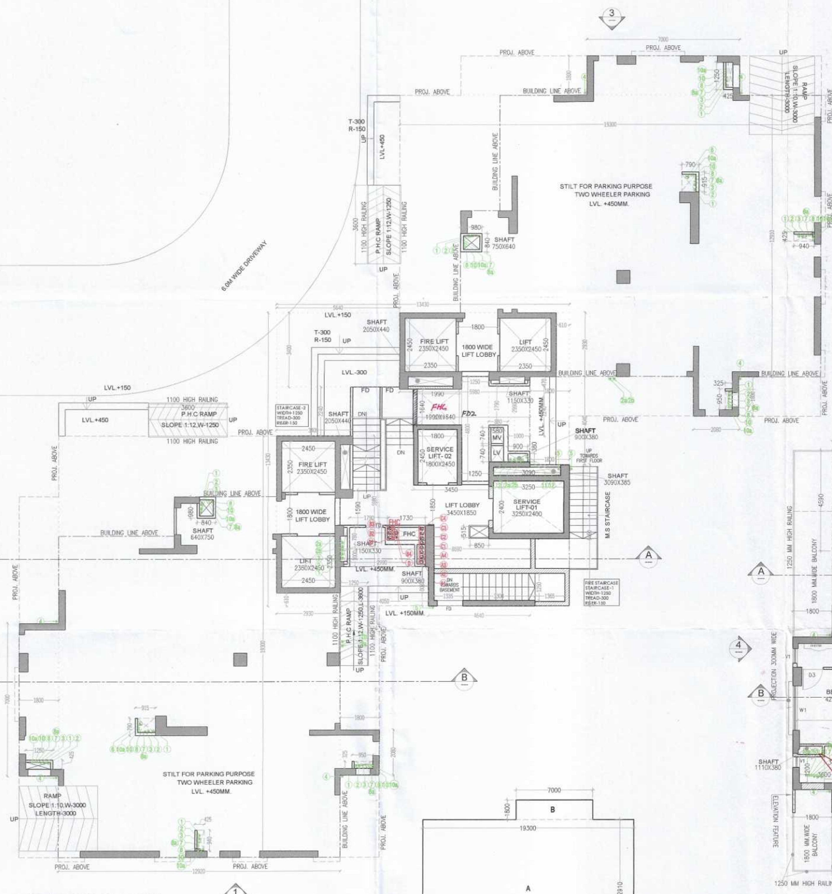
STILT / GROUND FLOOR PLAN
