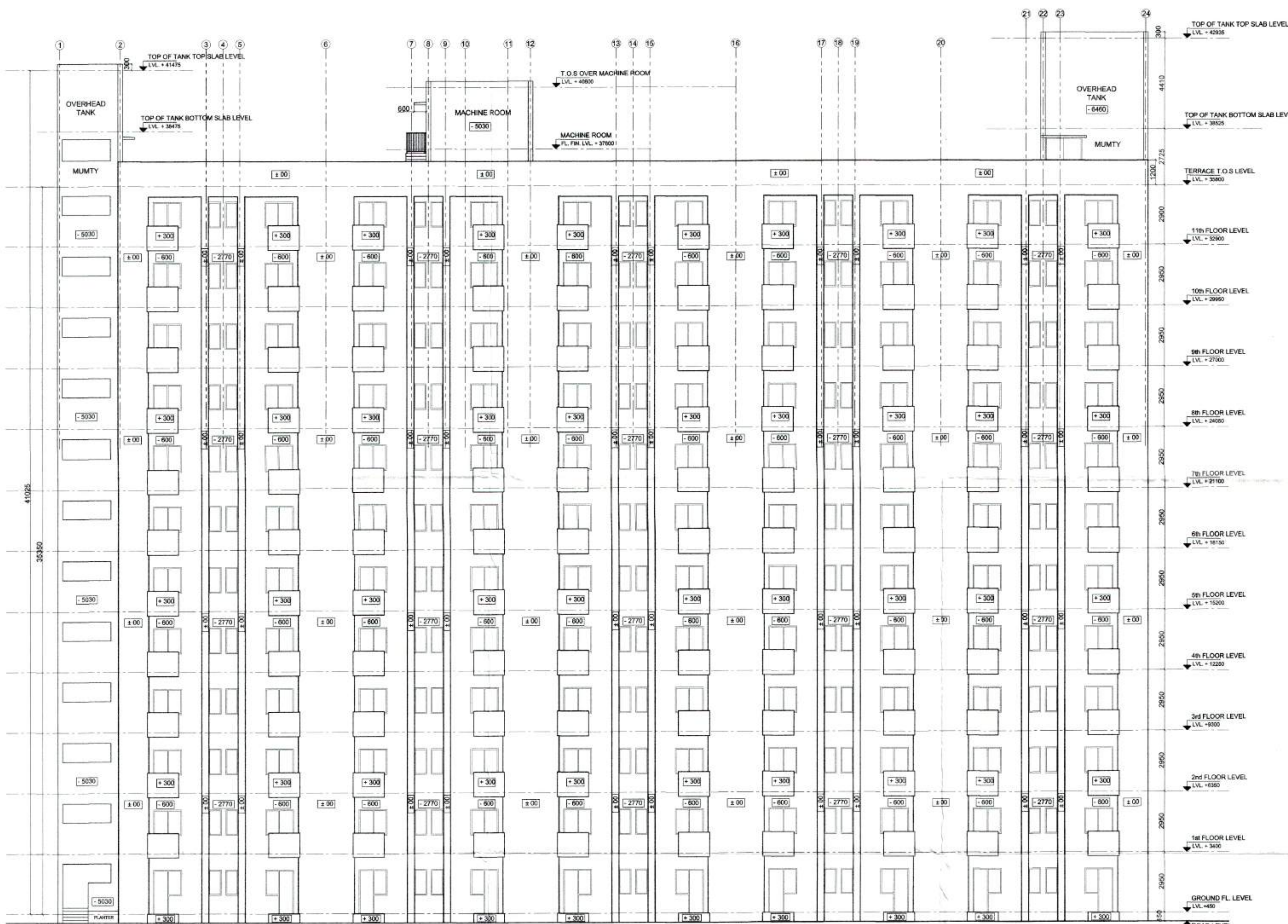
ELEVATION -E1 (EWS BLOCK)
