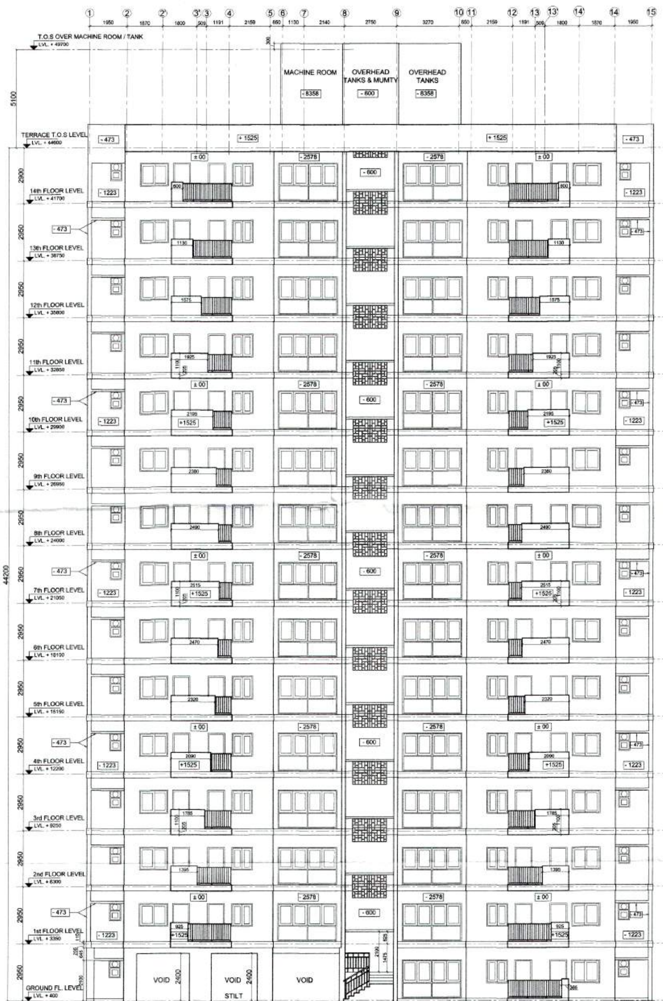
ELEVATION - 1 (TOWER T-10)
