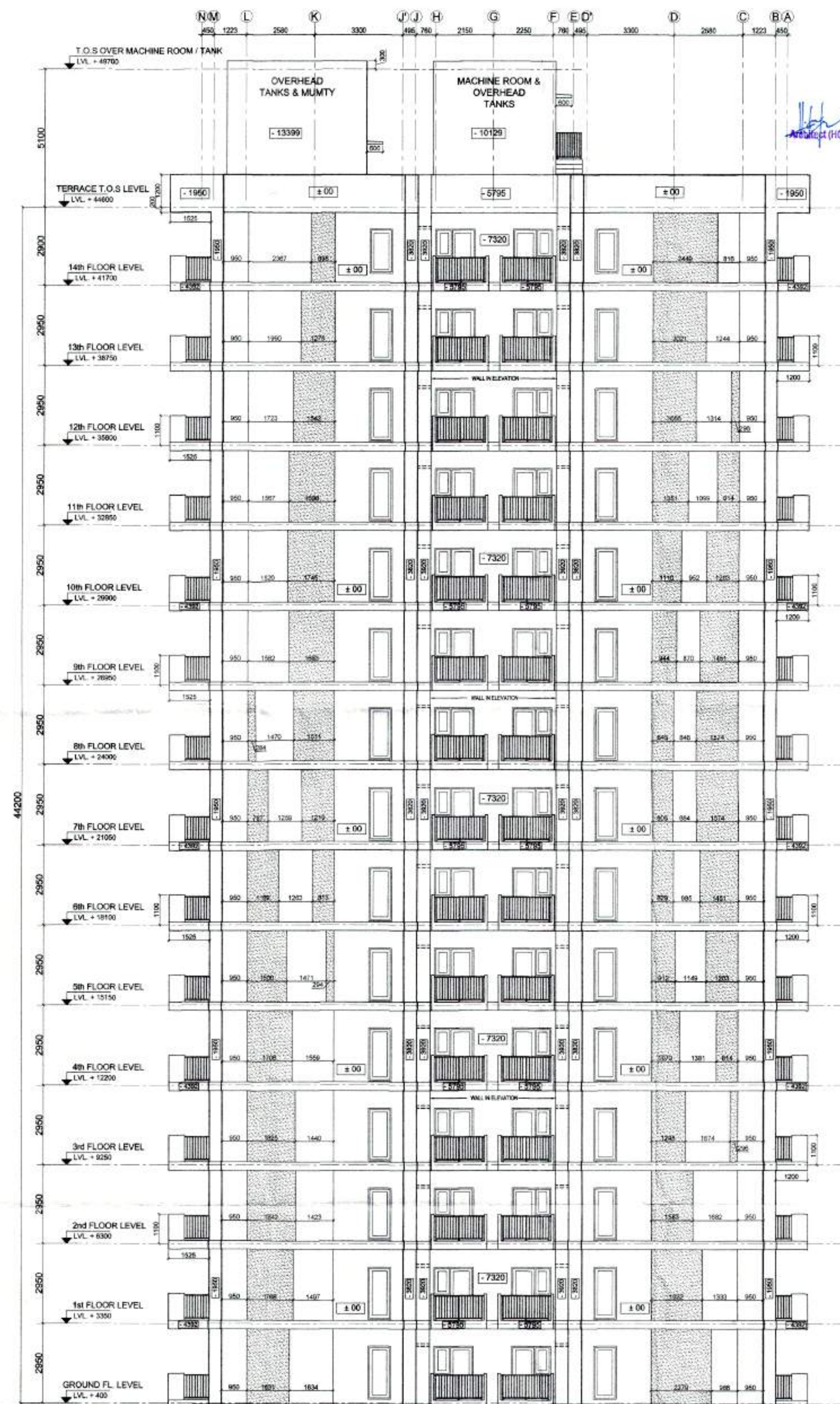
ELEVATION - 2 (TOWER T-10)
