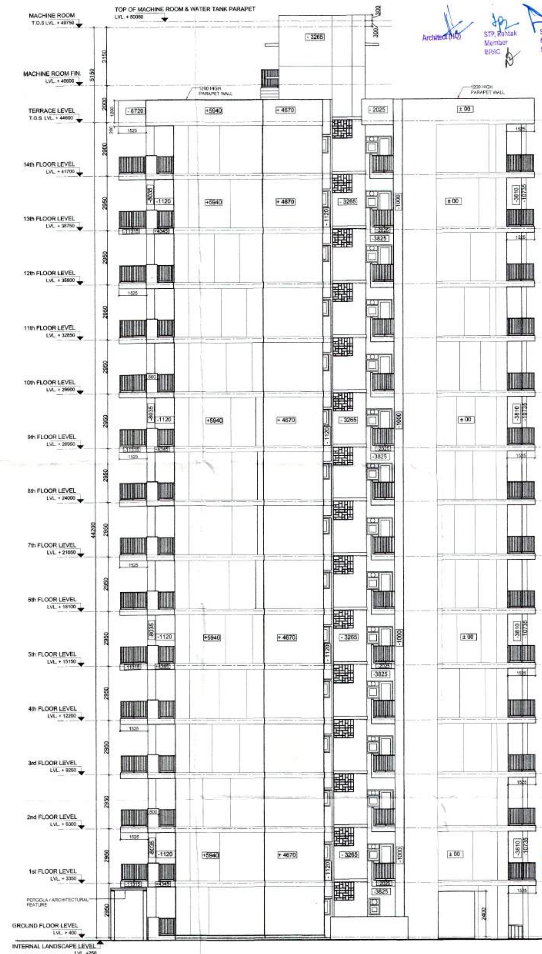
ELEVATION - 2 (For Towers T-8 & T-9)
