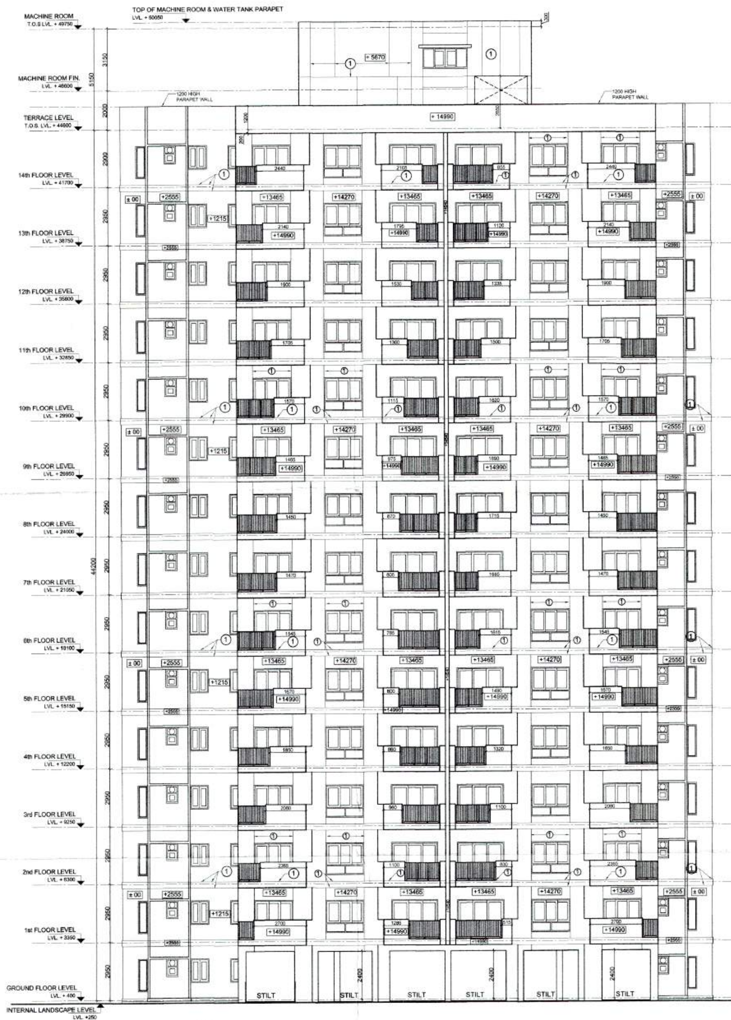
ELEVATION - 1 (For Towers T-8 & T-9)
