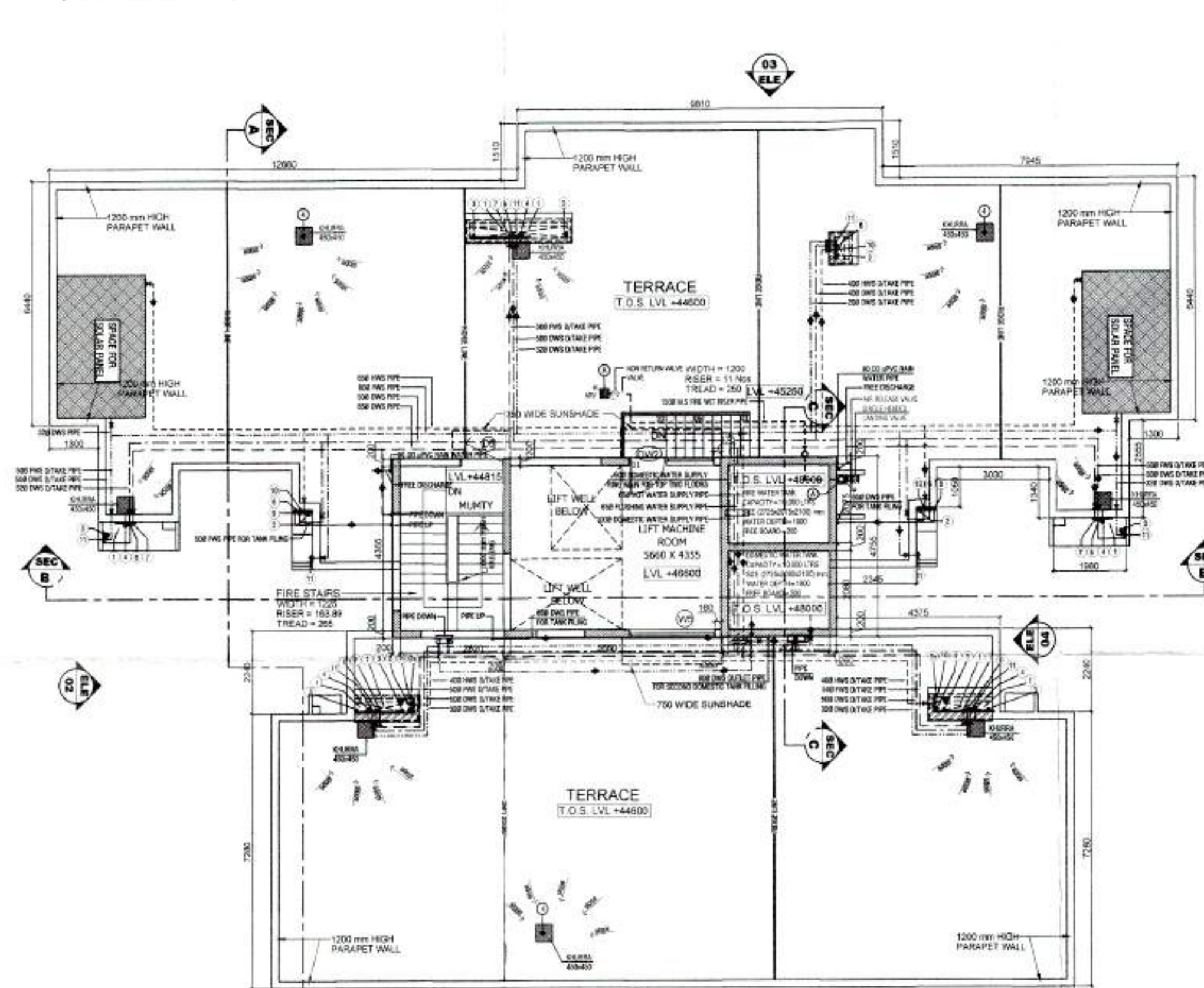
TERRACE PLAN (For Towers T-8 & T-9)
