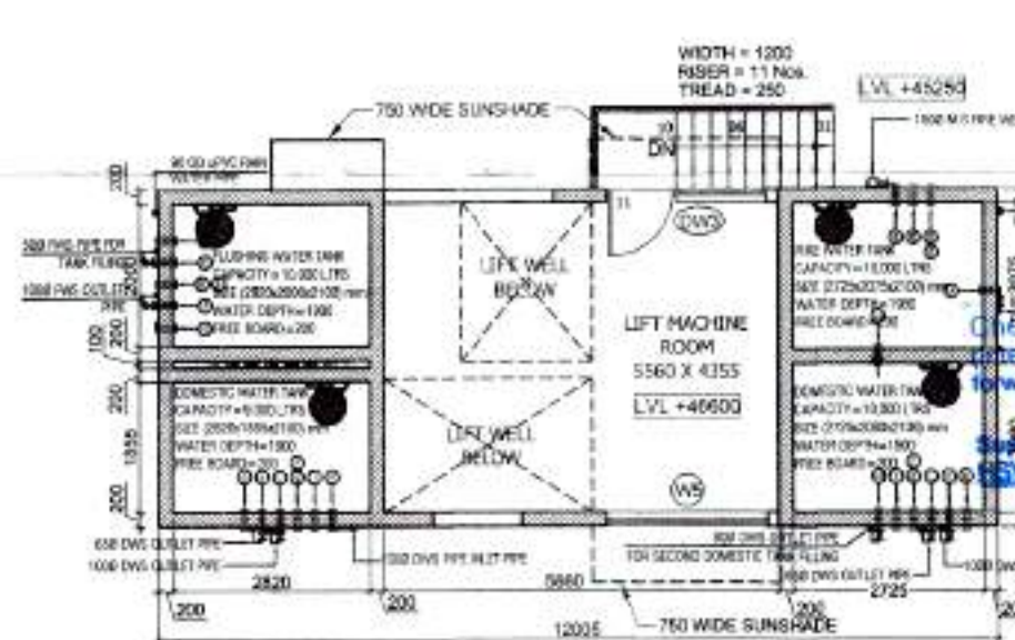
TANK & MACHINE ROOM LEVEL PLAN (For Towers T-8 & T-9)
