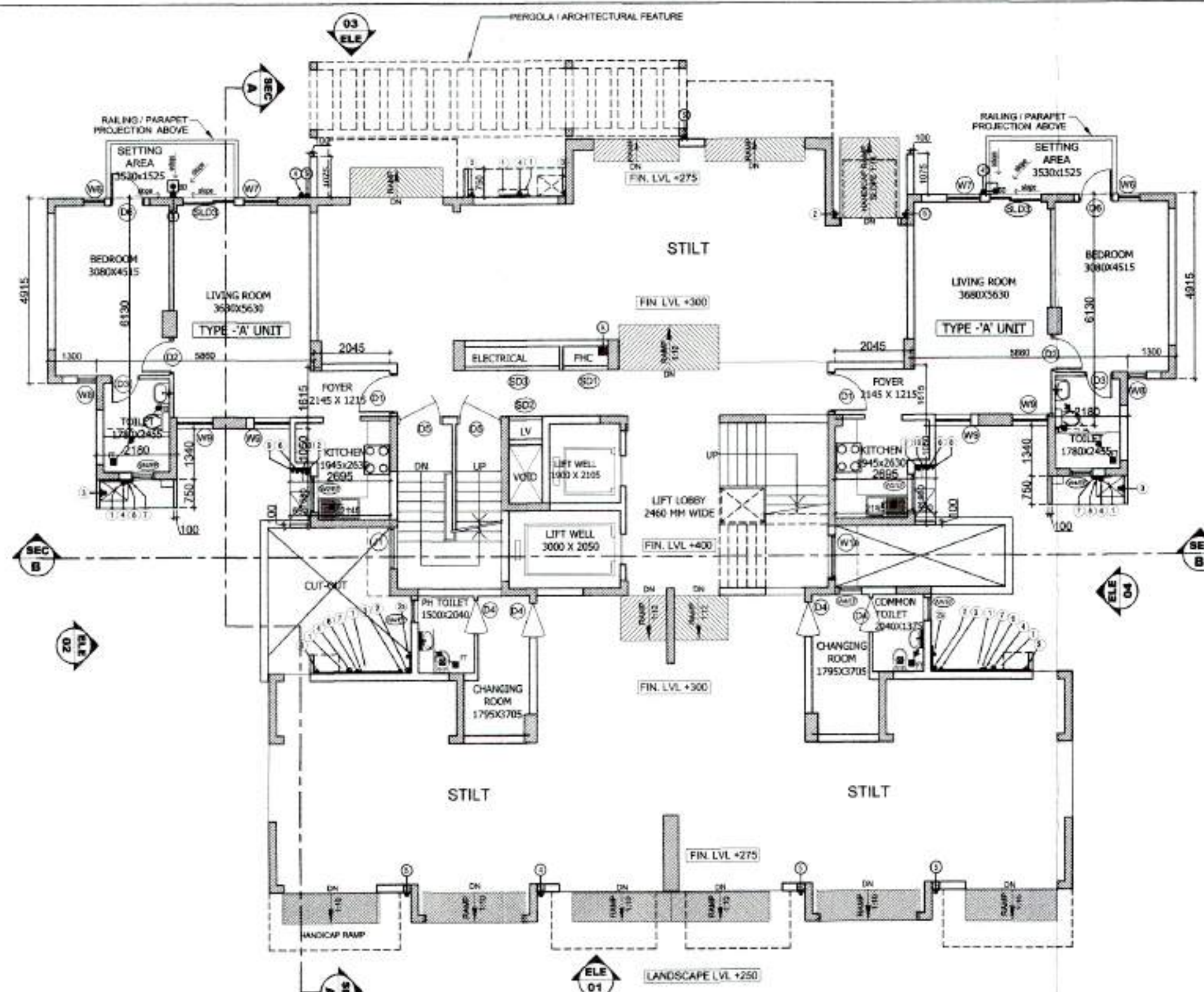
STILT/ GROUND FLOOR PLAN (For Tower T-9)
