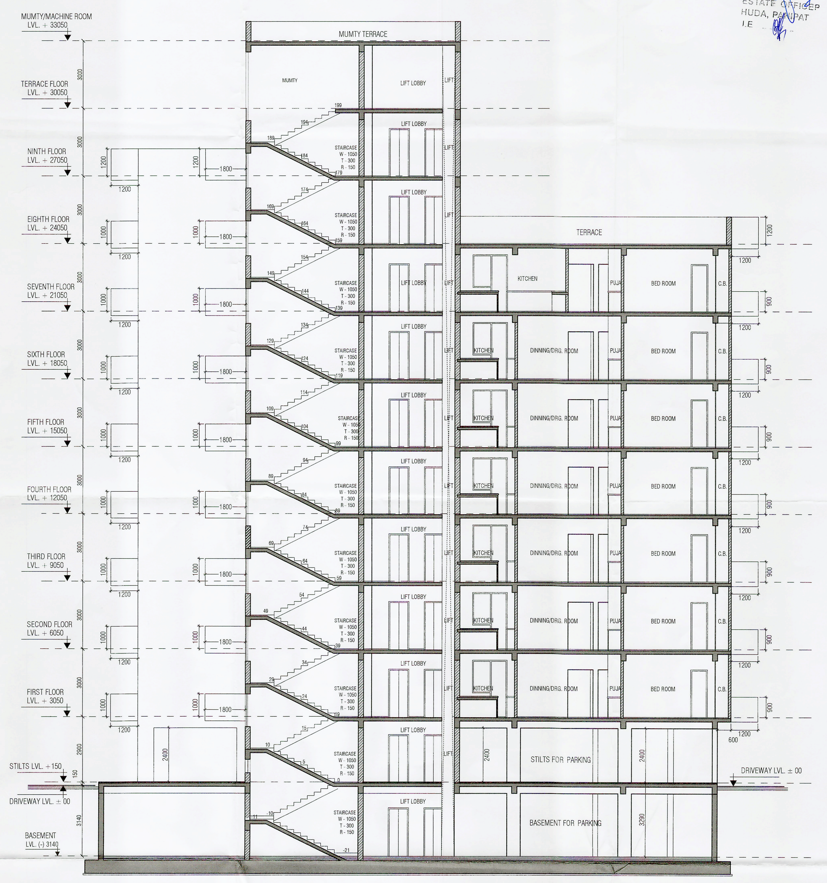
SECTION BB
