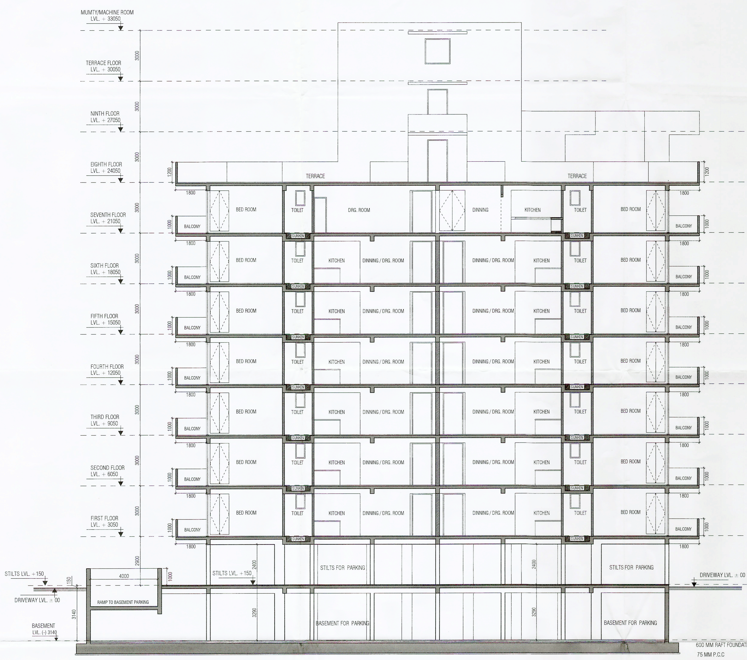
SECTION AA
