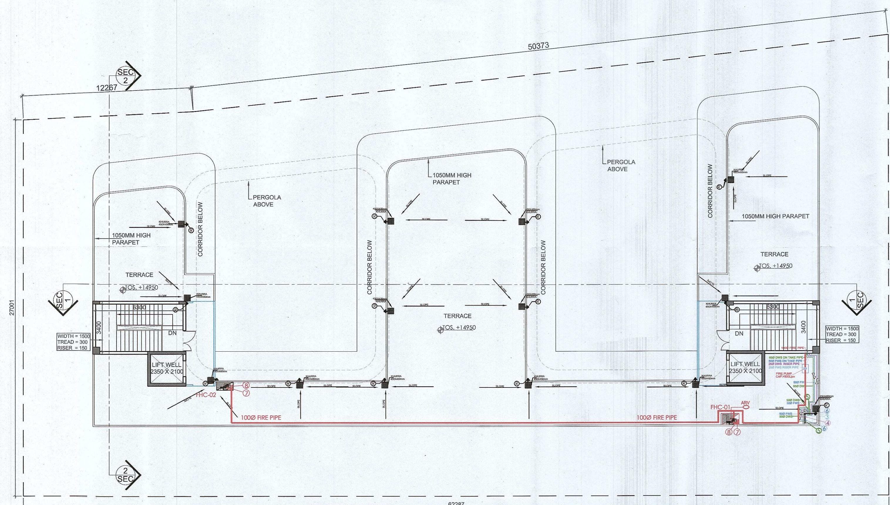
1 TERRACE PLAN SCALE 1:100
