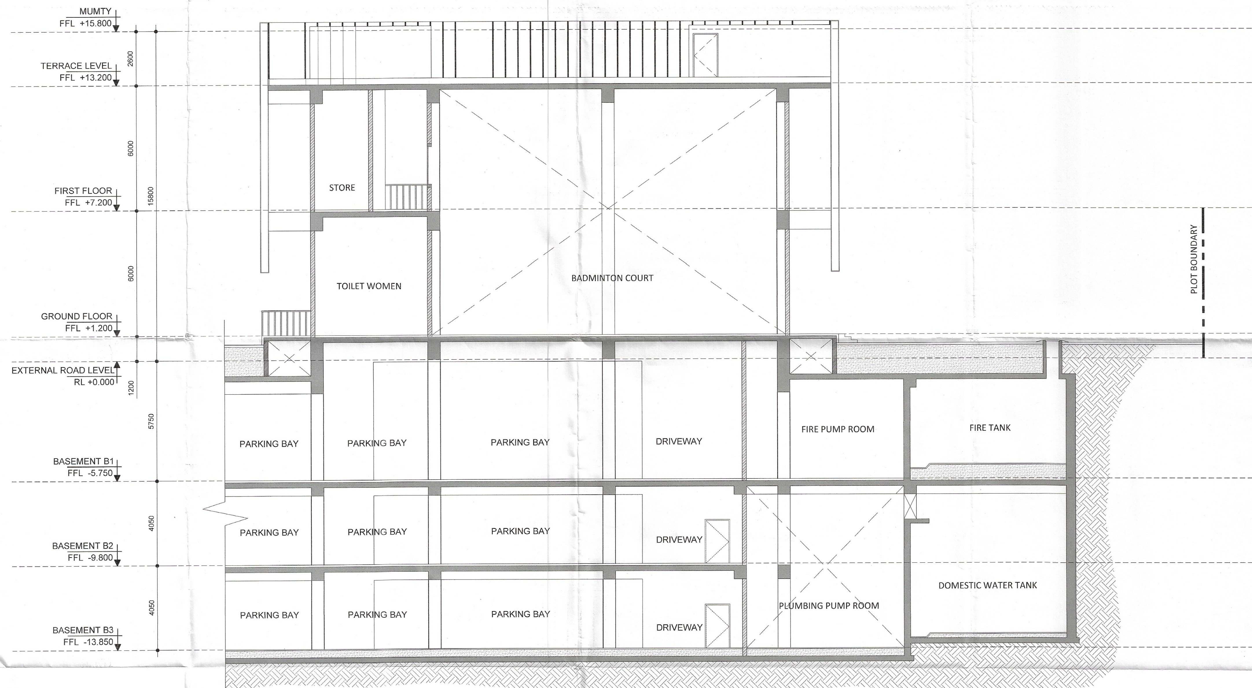
SECTION - B
