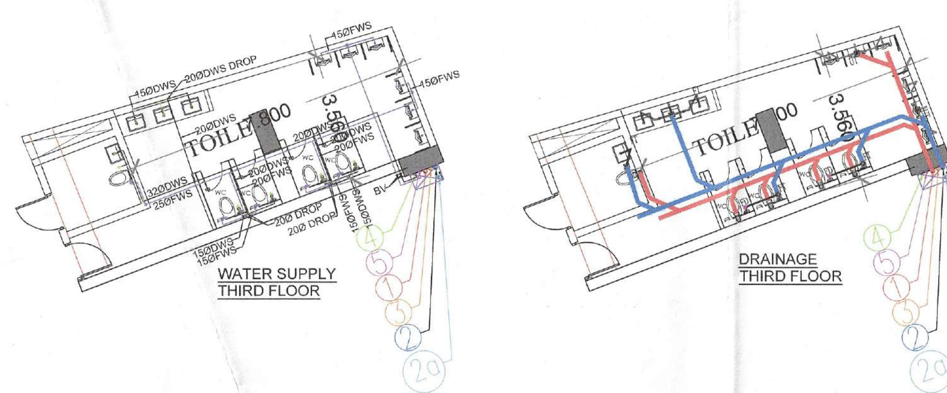
TOILET-2 SCALE - 1:100
