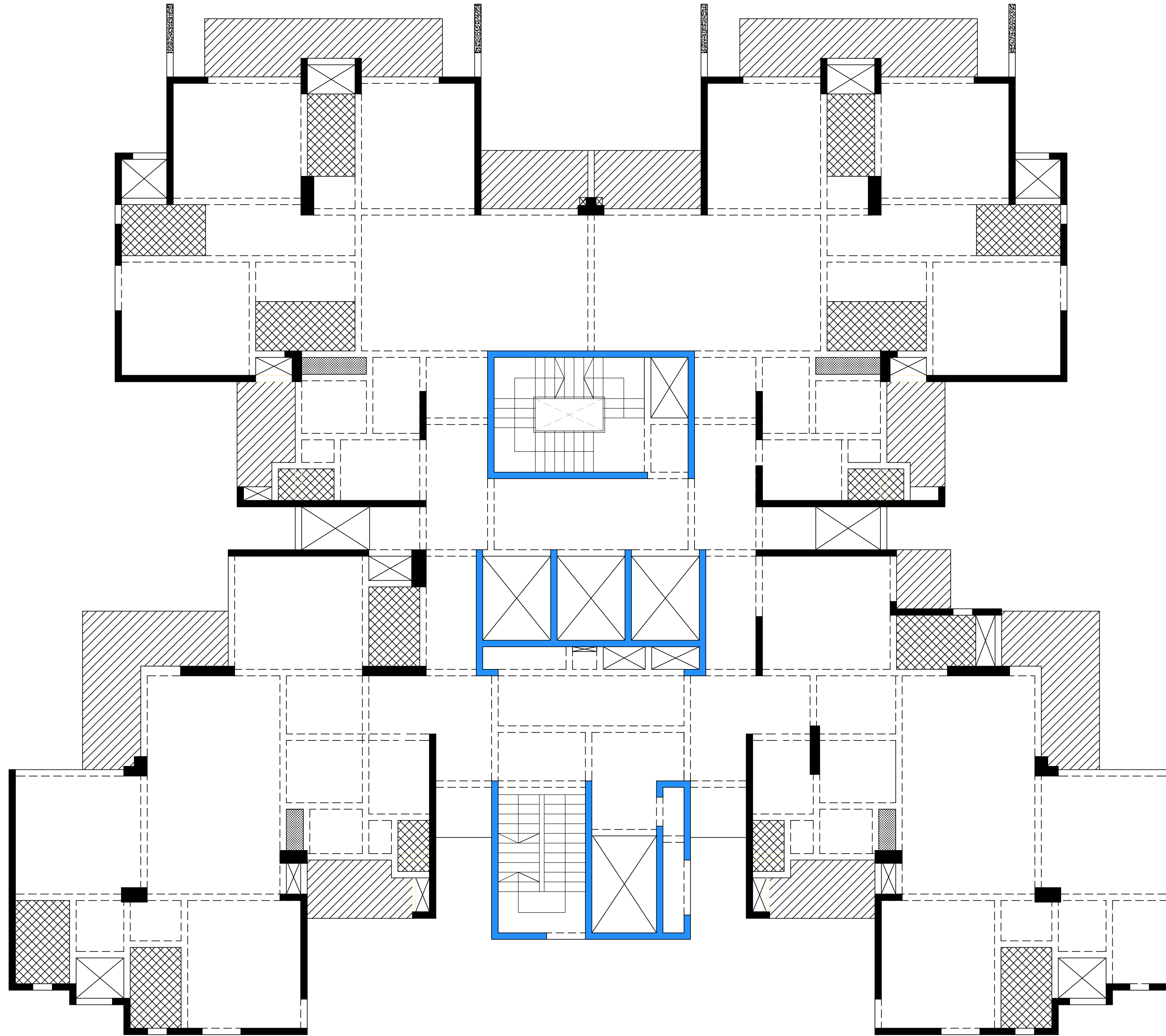
3RD FLOOR PLAN (POCKET-2)
