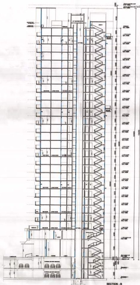
SECTION - B
