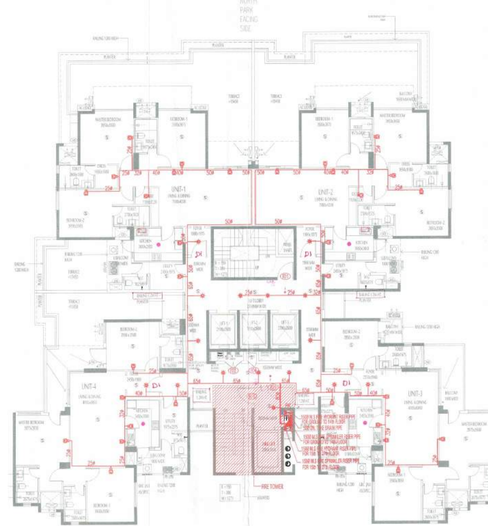
2ND FLOOR PLAN (POCKET-2)
