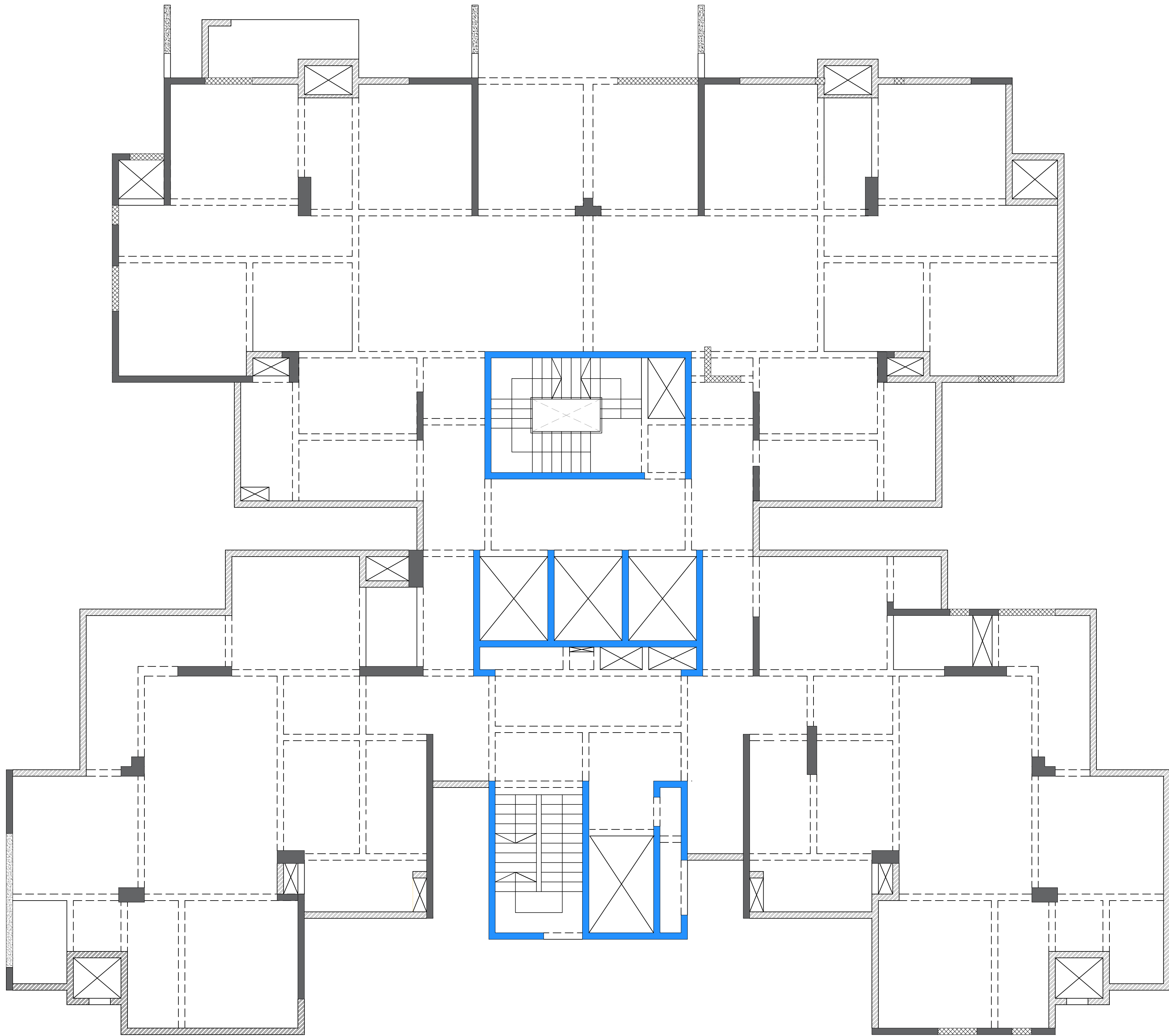
TERRACE LEVEL PLAN (POCKET-1)
