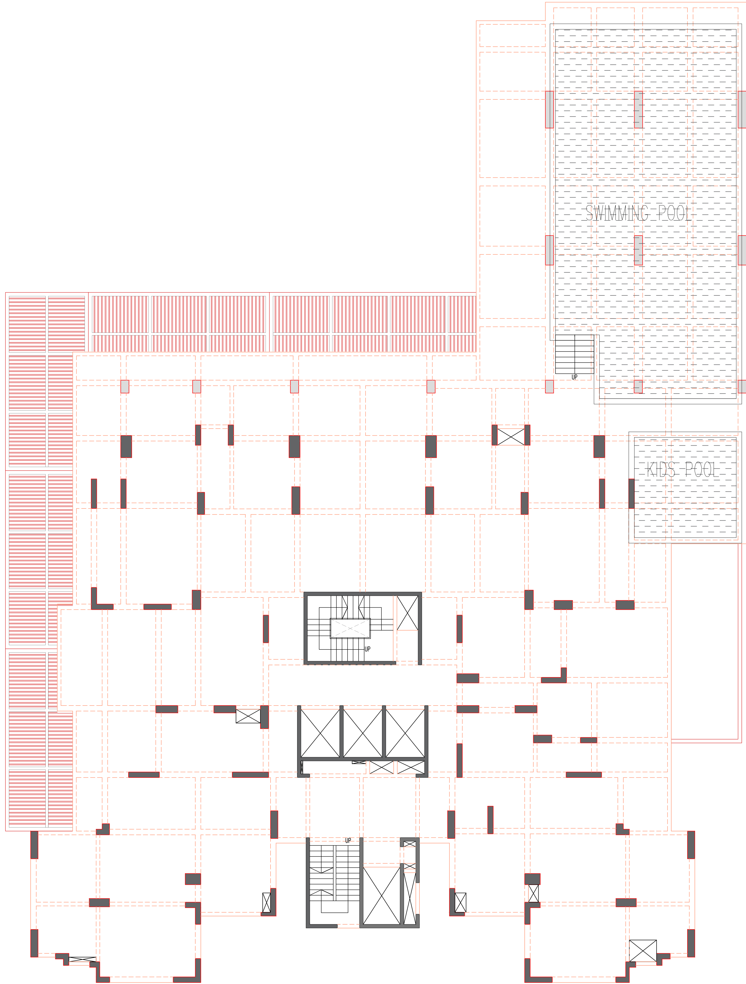
FIRST FLOOR LEVEL PLAN ALL BEAMS ARE 200x600 / 250x600 / 450x600mm U.N.O
