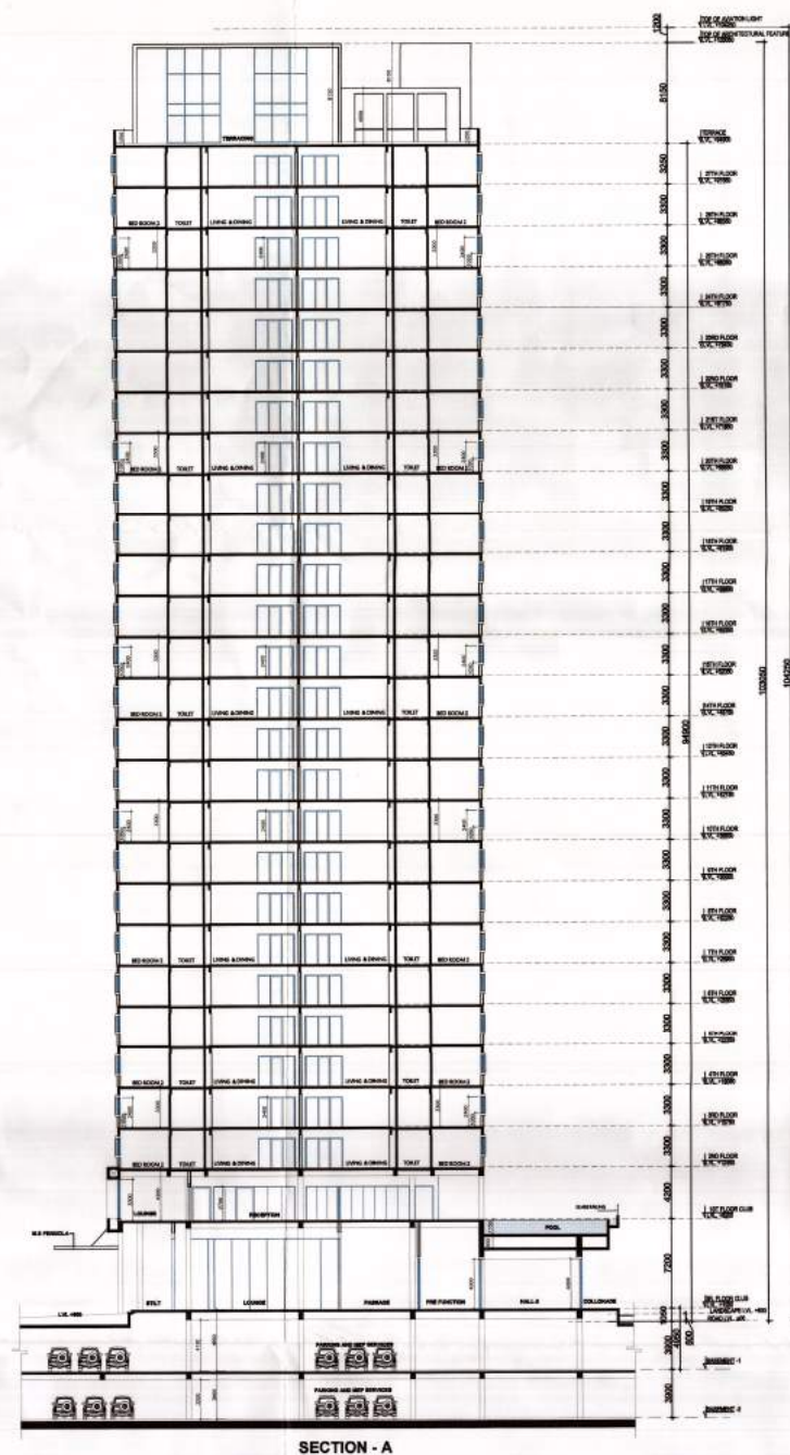
SECTION - A
