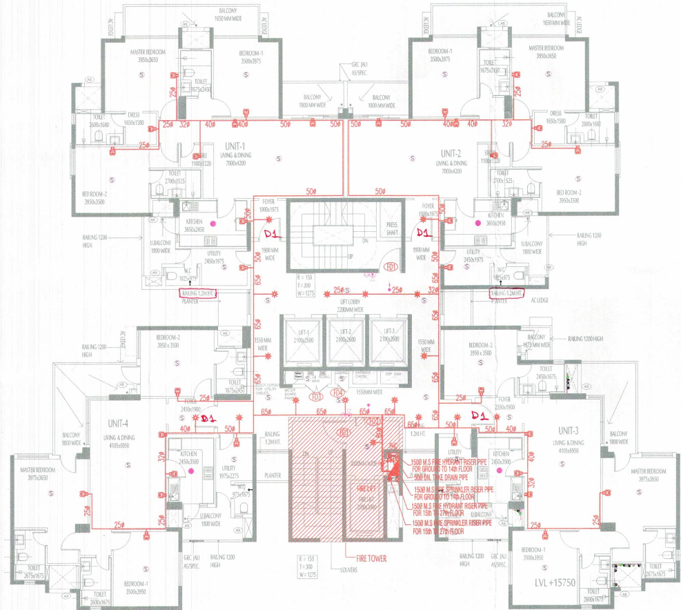
3RD FLOOR PLAN (POCKET-1)
