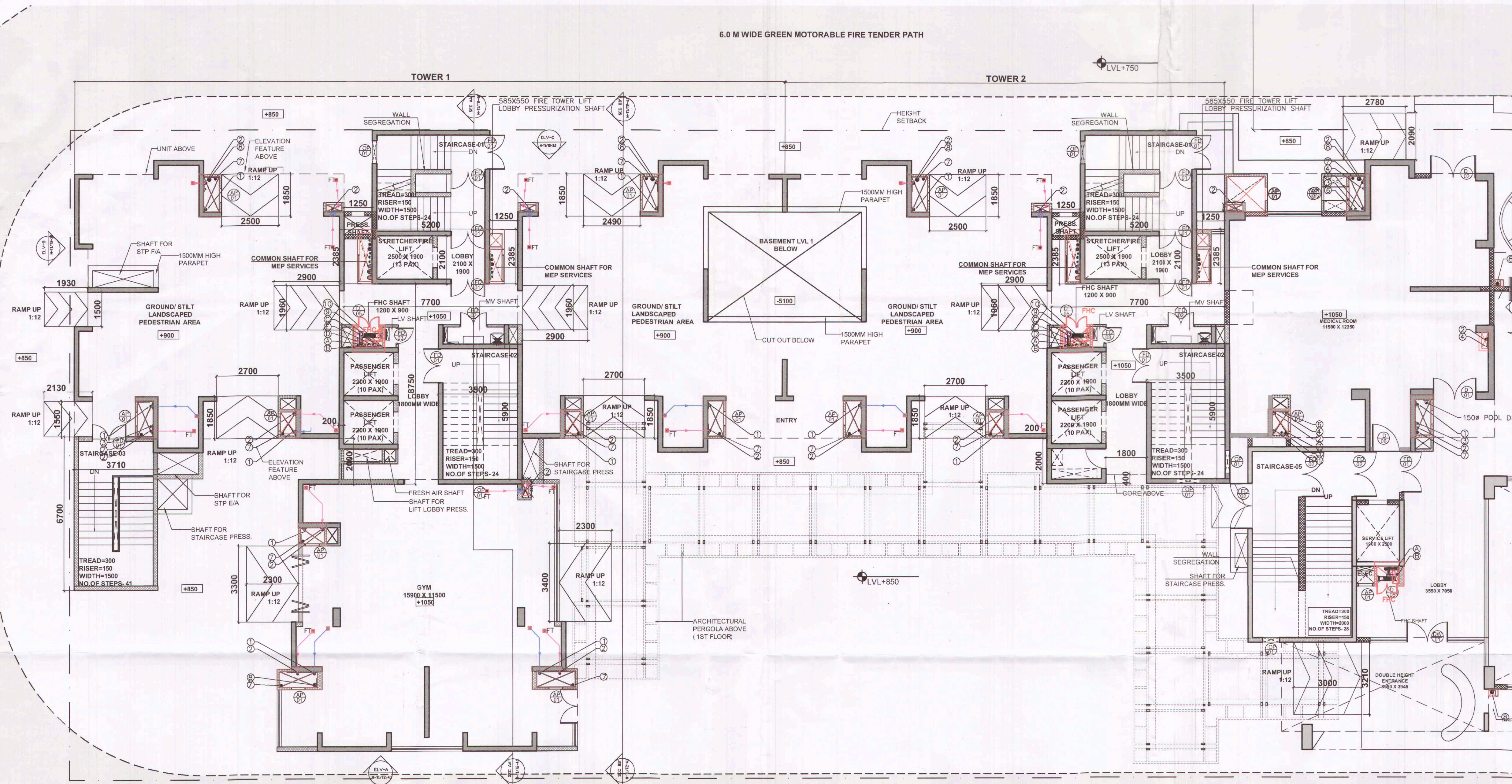
GROUND/STILT FLOOR PLAN
