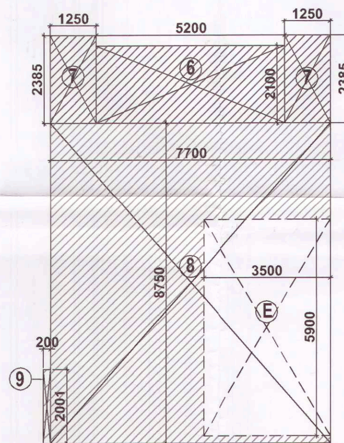
GROUND/STILT FLOOR- FAR CALCULATION PLAN
