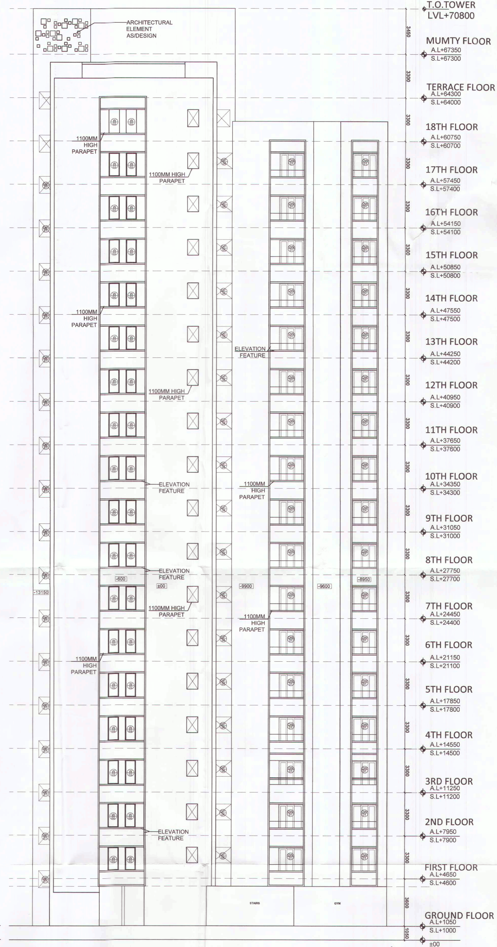
ELEVATION-B
