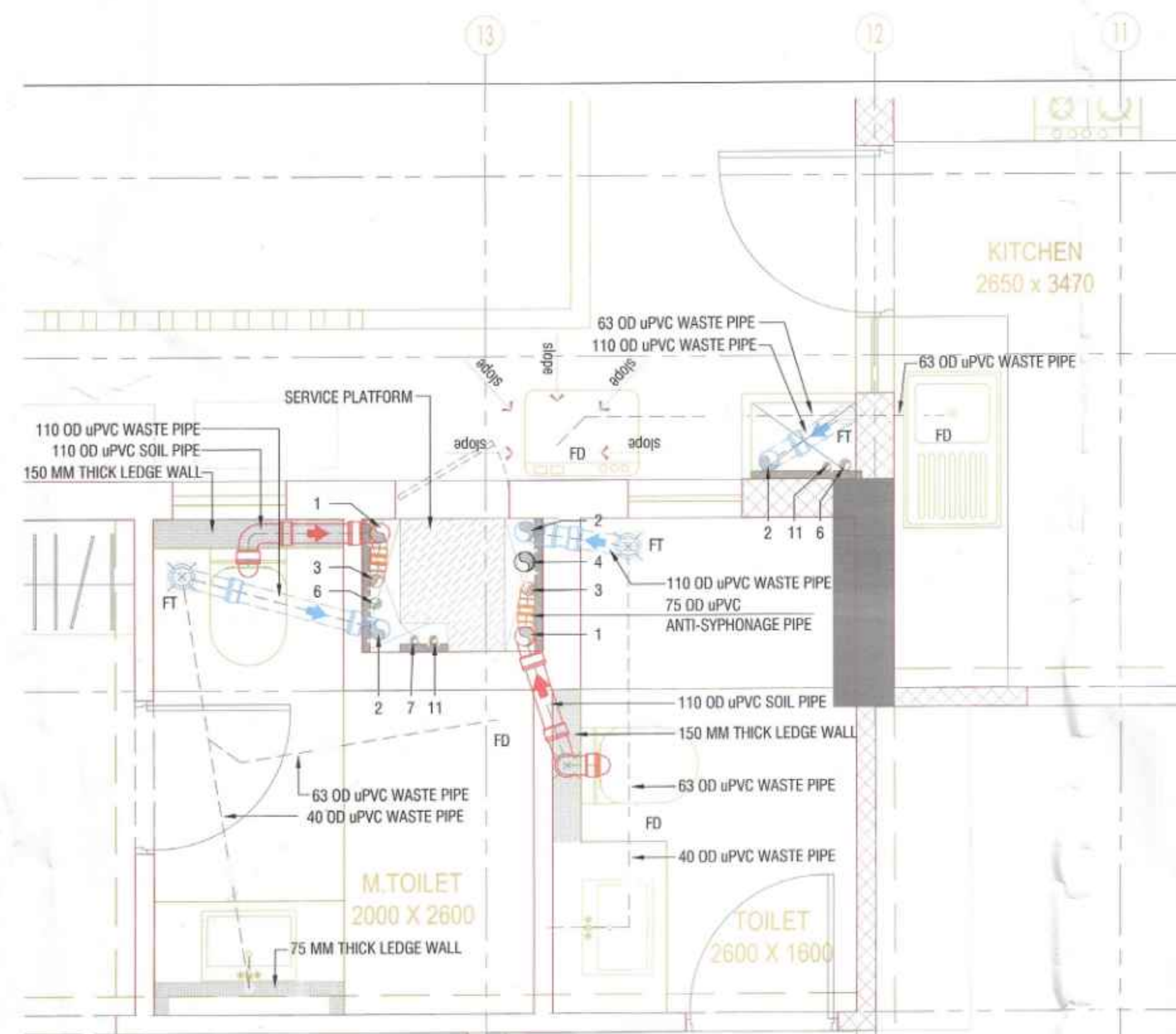
TYPICAL FLOOR M.TOILET (2000x2600), TOILET(2600x1600) & KITCHEN (2650x3470) DRAINAGE LAYOUT
