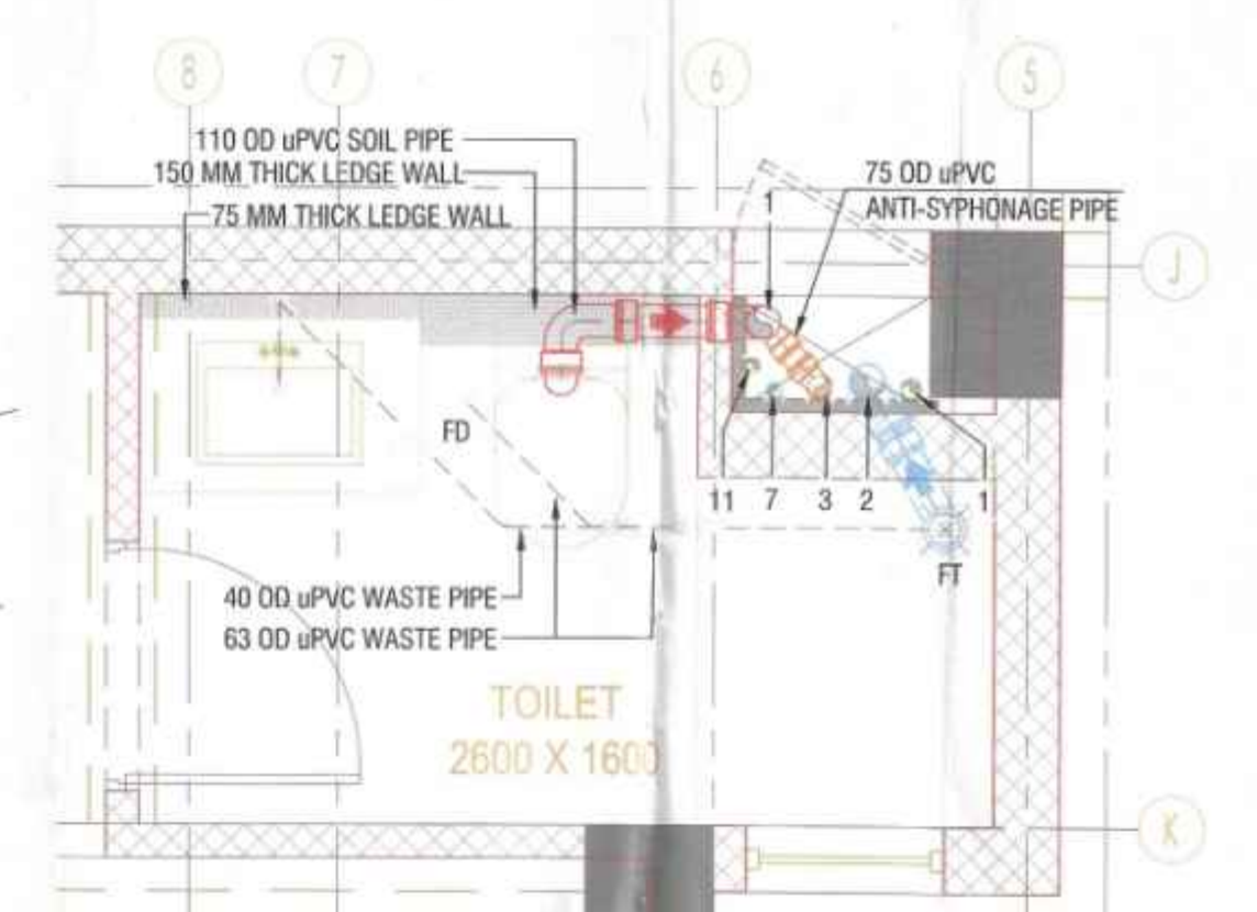
TYPICAL FLOOR TOILET (2600x1600) DRAINAGE LAYOUT
