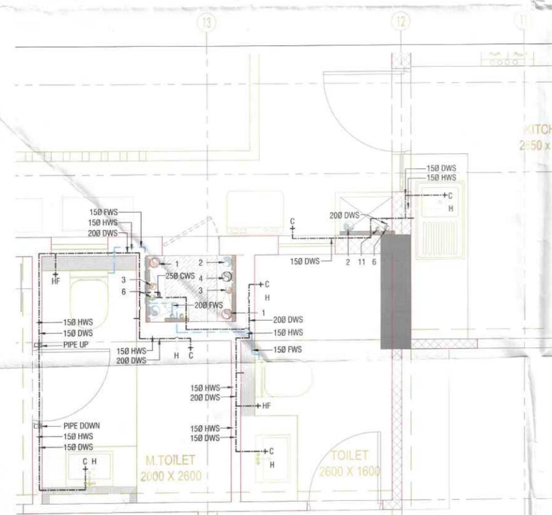
TYPICAL FLOOR M.TOILET (2000x2600), TOILET(2600x1600) & KITCHEN (2650x3470) DRAINAGE LAYOUT
