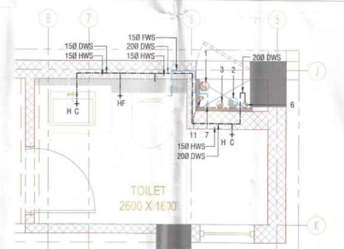
TYPICAL FLOOR TOILET (2600x1600) WATER SUPPLY LAYOUT
