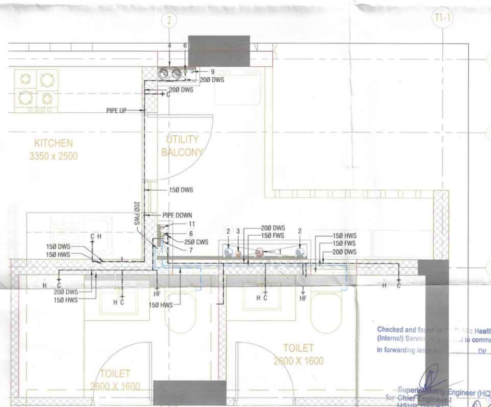
TYPICAL FLOOR TOILET (2600x1600) & KITCHEN (3350x2500) WATER SUPPLY LAYOUT
