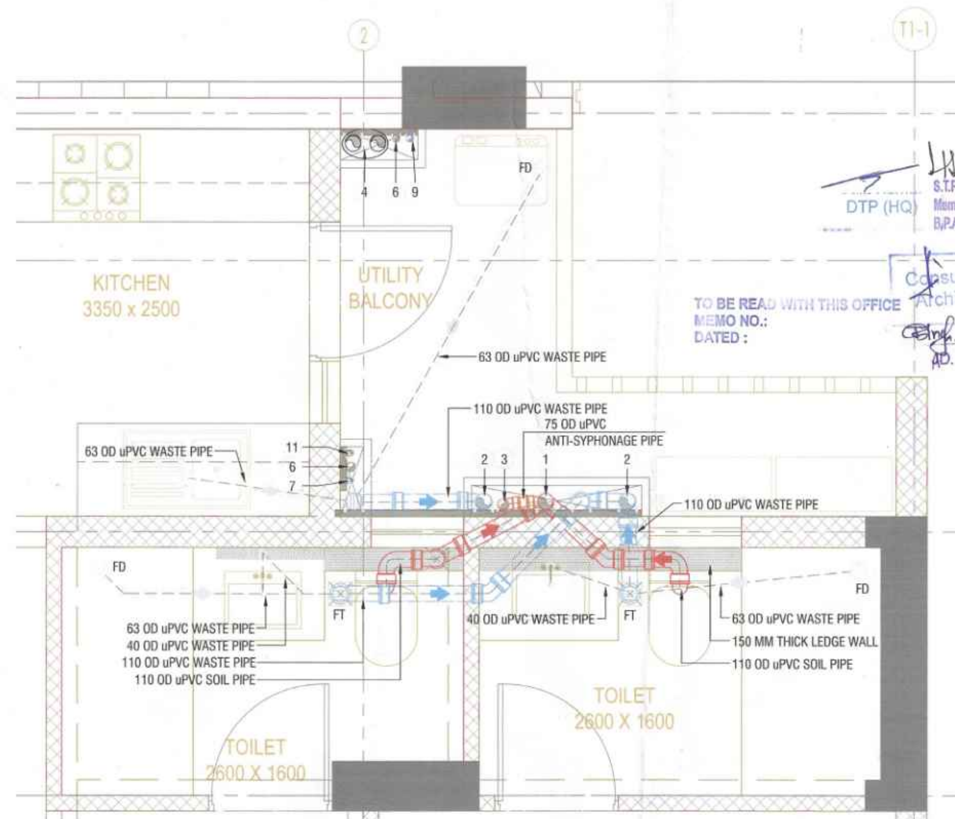
TYPICAL FLOOR TOILET (2600x1600) & KITCHEN (3350x2500) DRAINAGE LAYOUT
